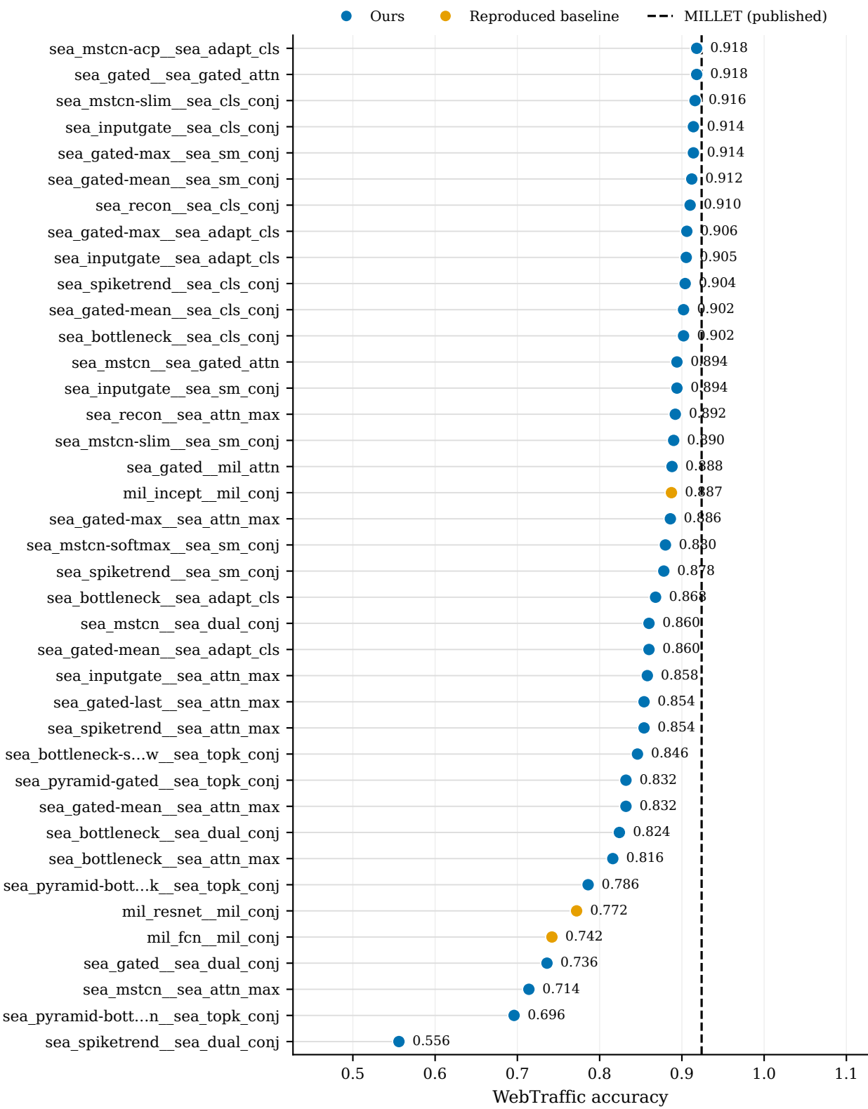
Accuracy &lt; 0.92 (39 models)
