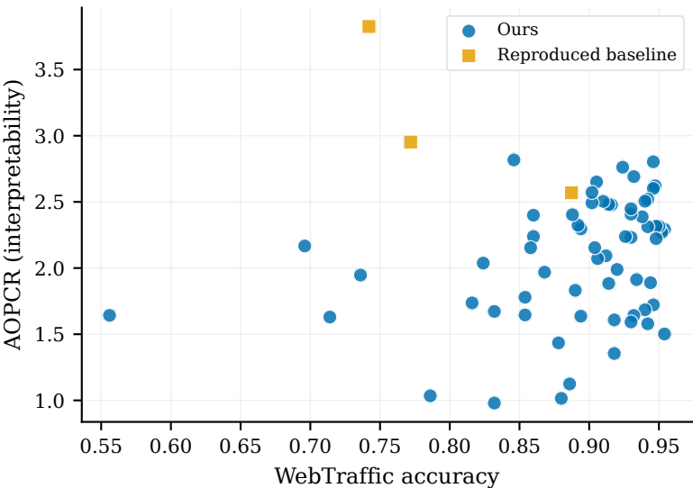
Accuracy vs AOPCR (Spearman \rho = 0.19 )
