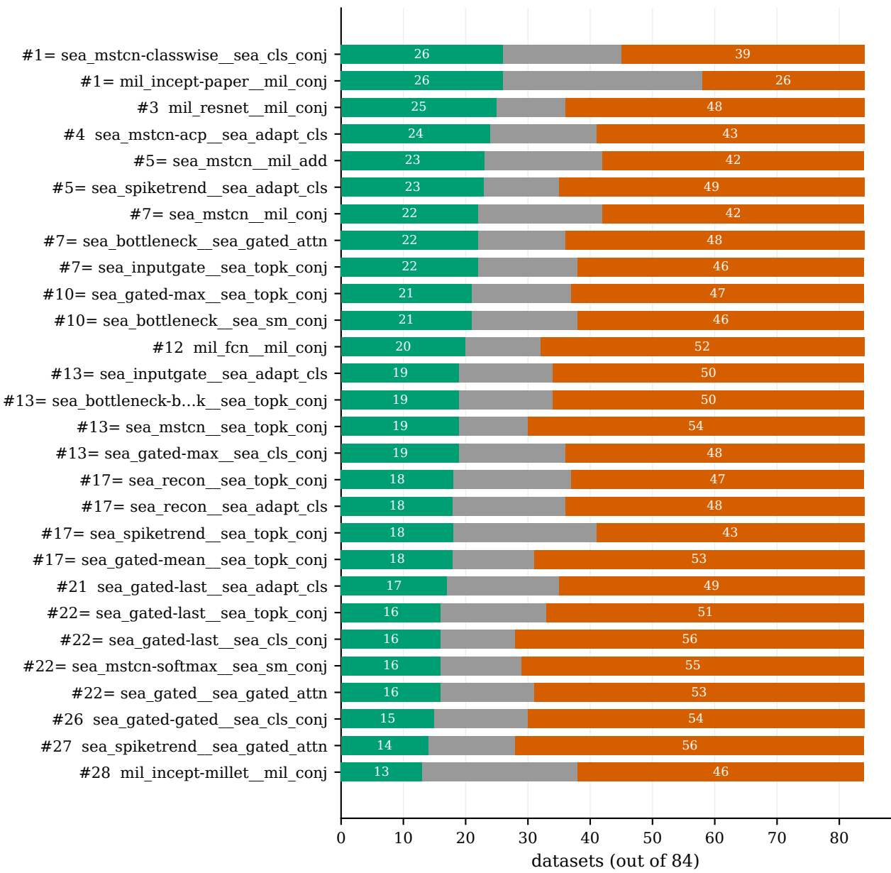
Win / tie / loss vs MILLET (accuracy)
