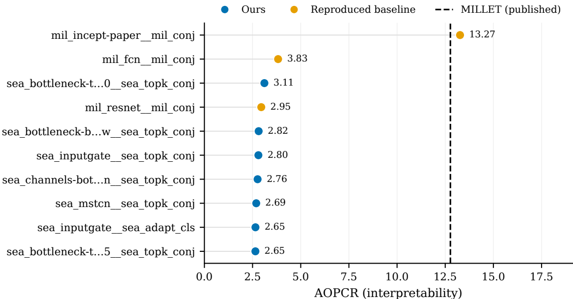
WebTraffic: AOPCR (top 10)
