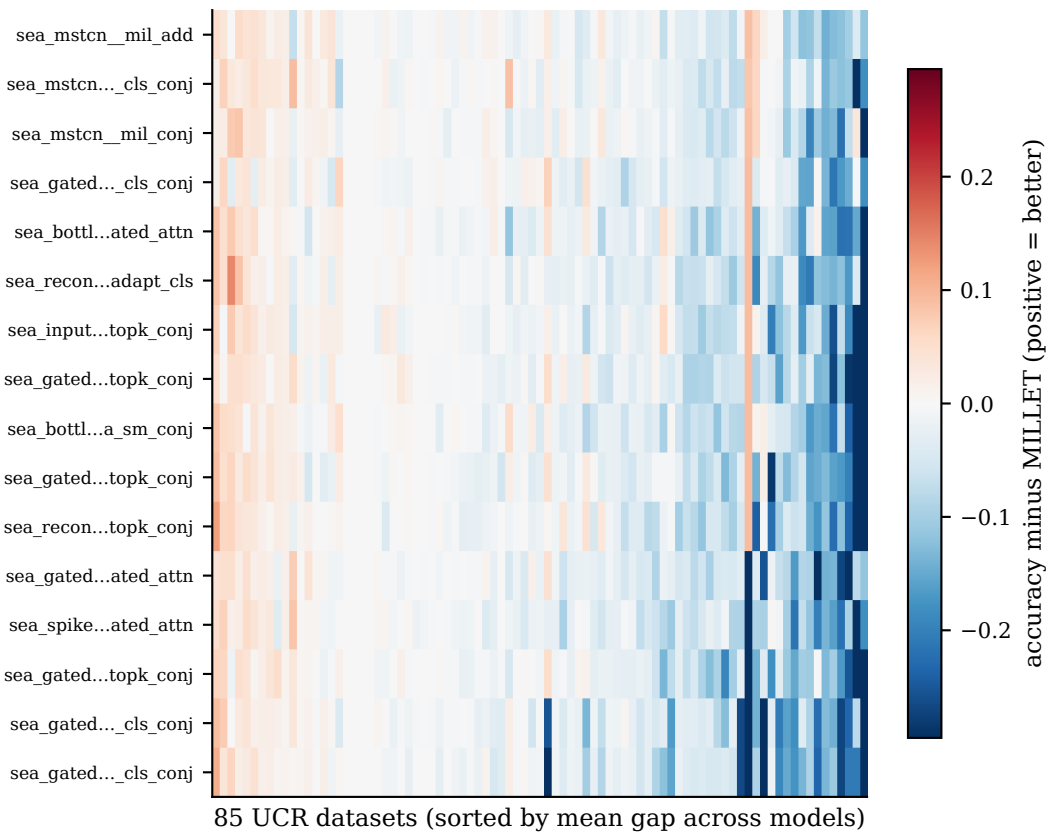
Per-dataset accuracy against MILLET
