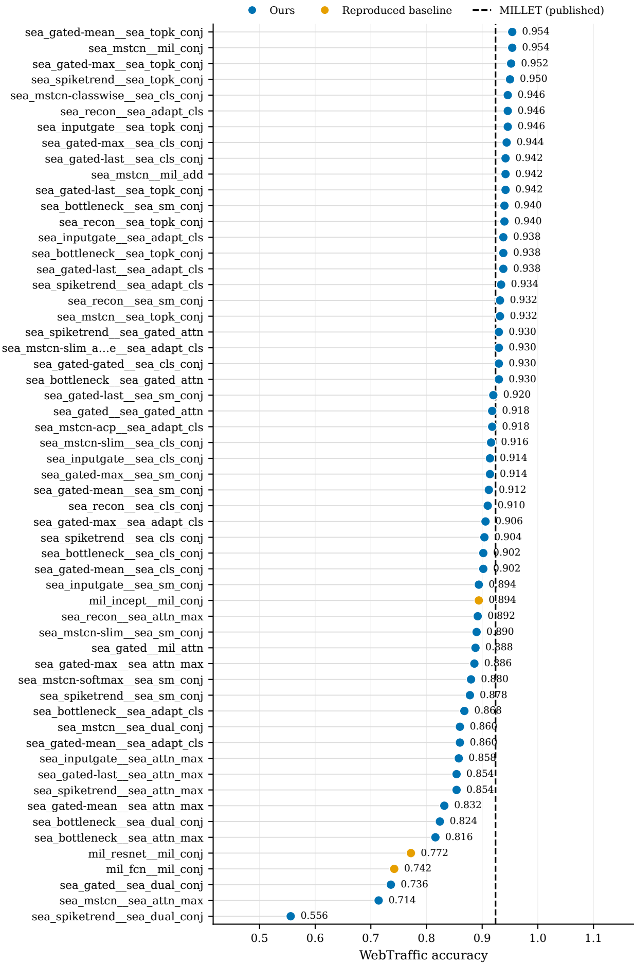
WebTraffic: Accuracy (all 57 models)
