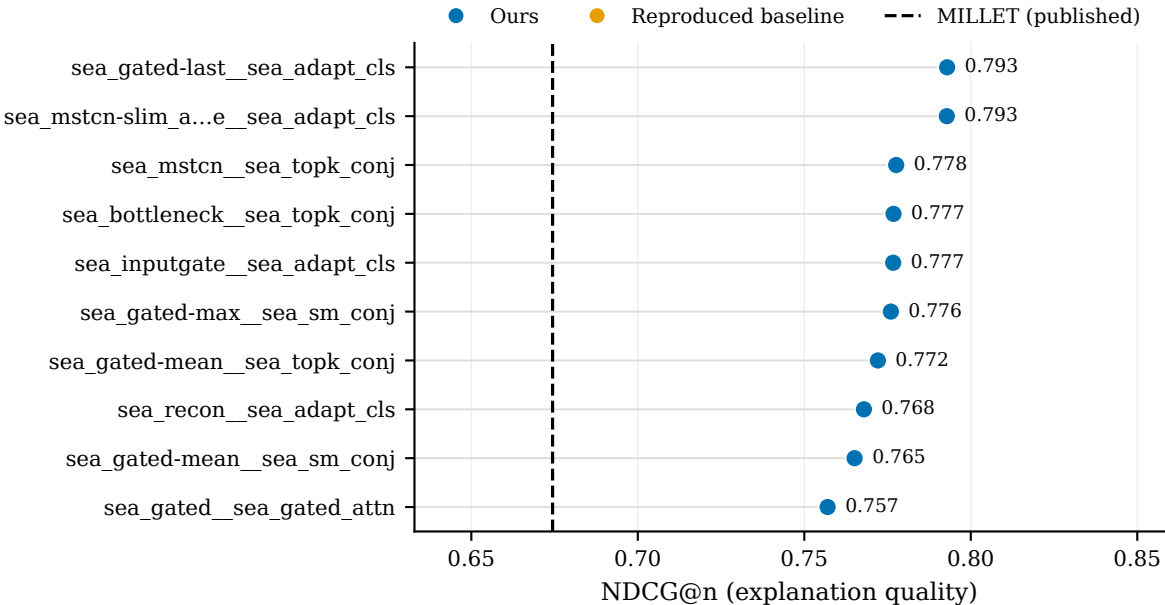
WebTraffic: NDCG@n (top 10)
