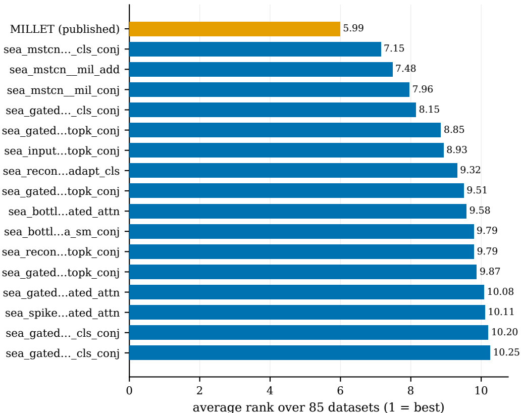
Average rank (accuracy)
