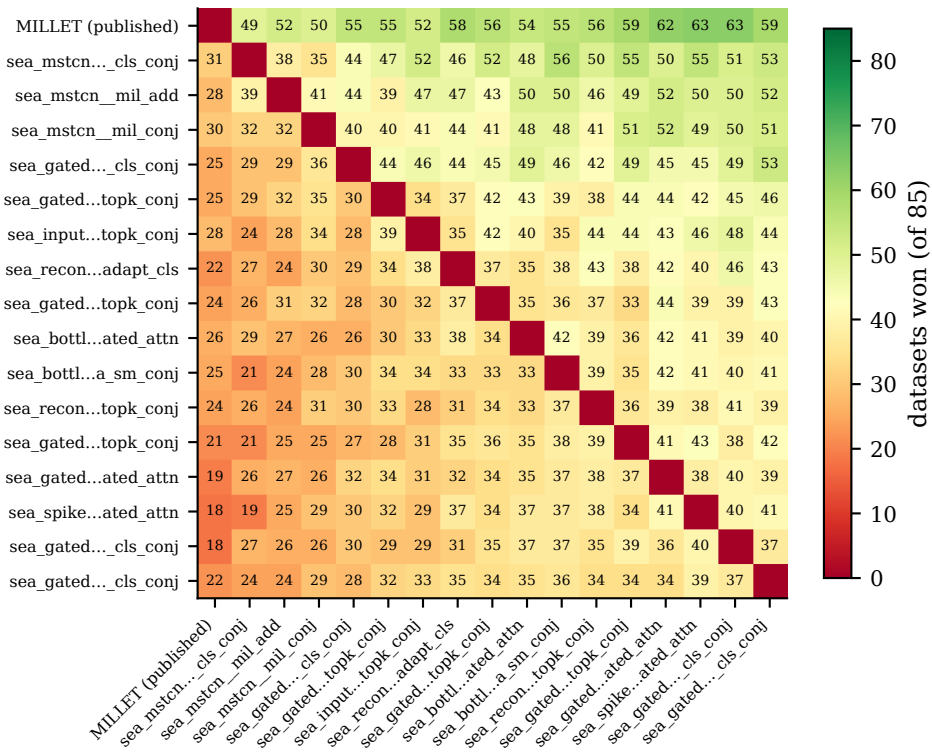
Head-to-head wins (accuracy) row beats column on this many datasets
