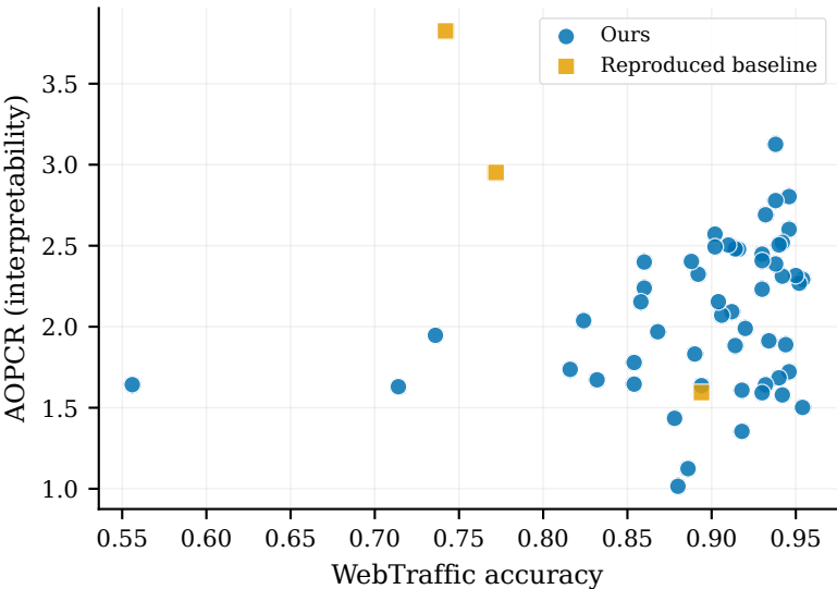
Accuracy vs AOPCR (Spearman \rho = 0.20 )
