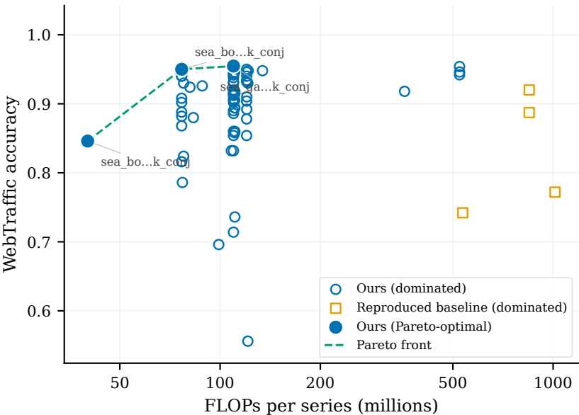
Accuracy vs FLOPs
