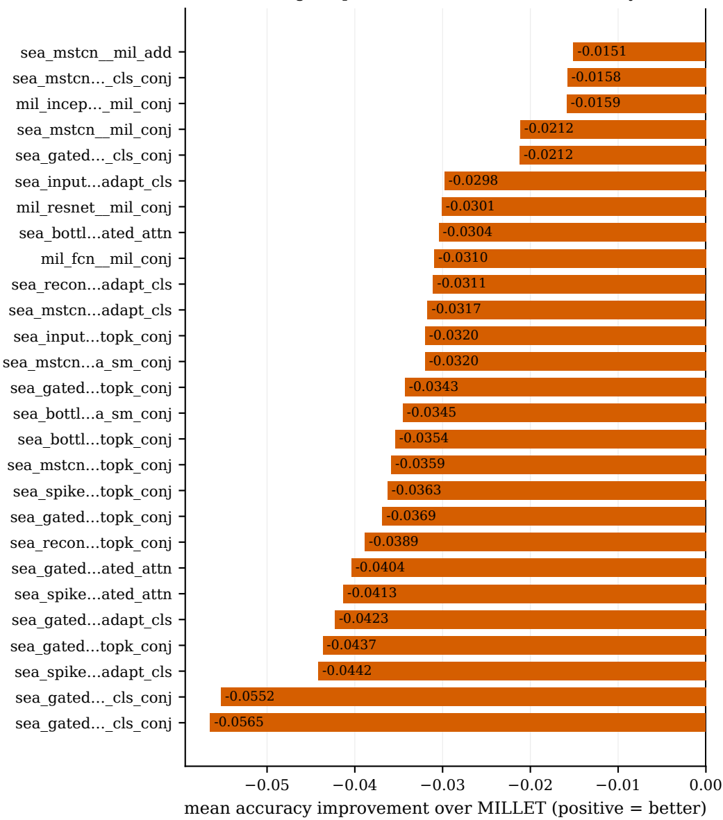
Average improvement over MILLET (accuracy)
