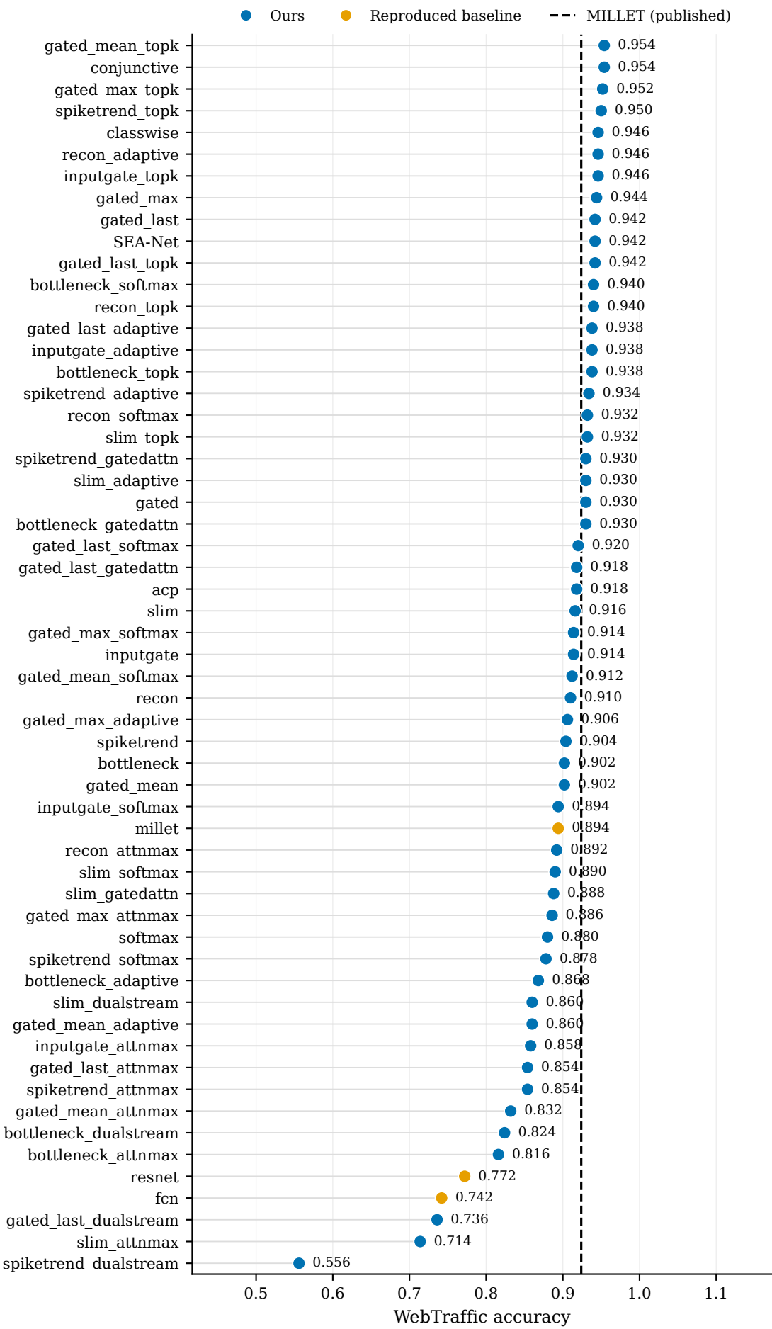
WebTraffic: Accuracy (all 57 models)
