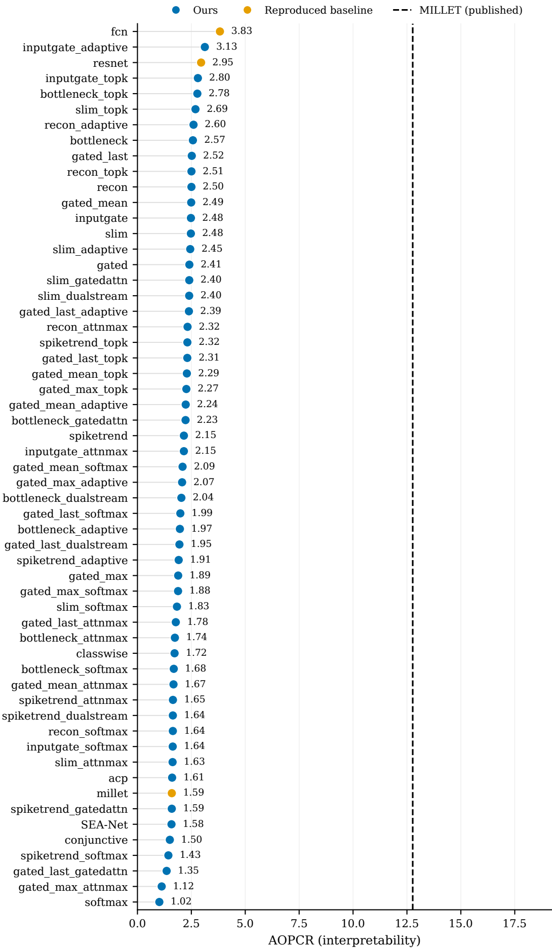
WebTraffic: AOPCR (all 57 models)
