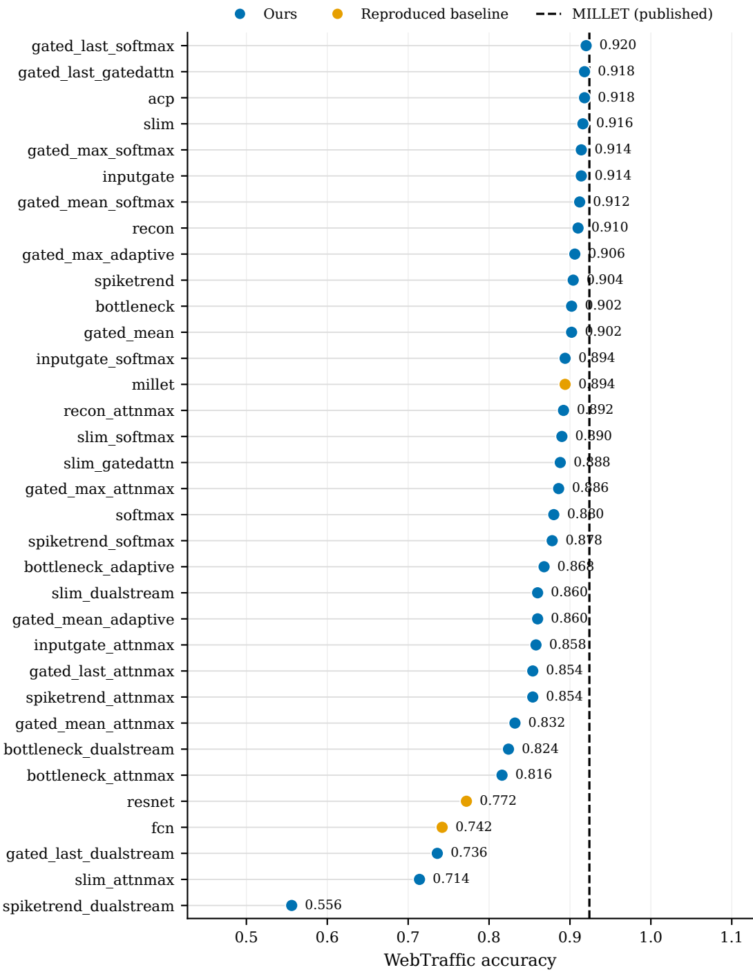
Accuracy &lt; 0.93 (34 models)
