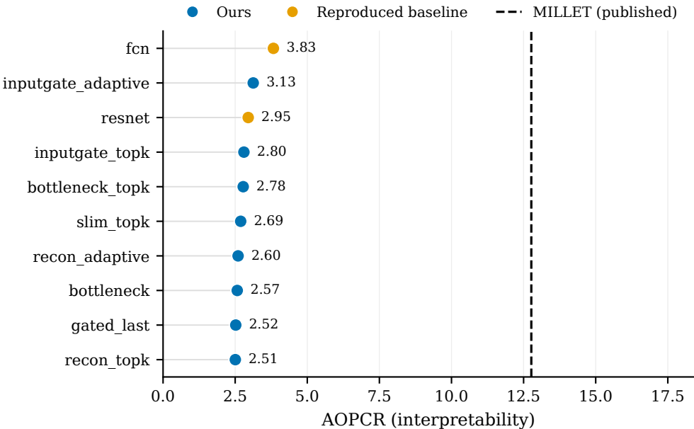
WebTraffic: AOPCR (top 10)
