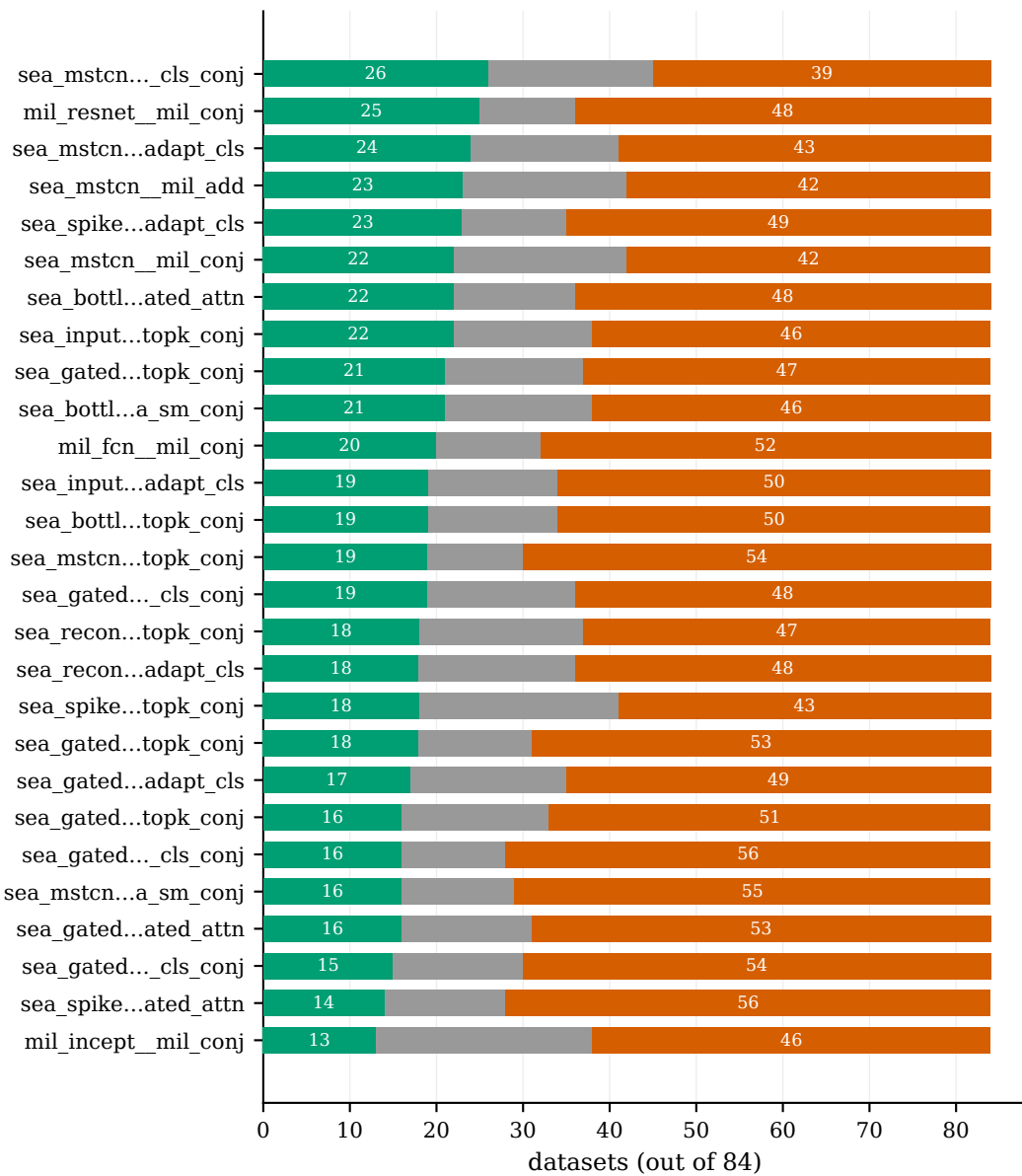
Win / tie / loss vs MILLET (accuracy)
