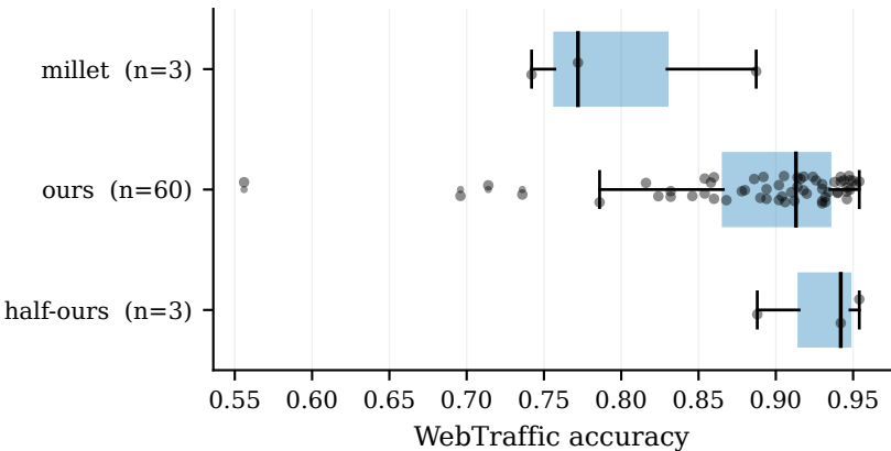
Accuracy by how much of the model is new
