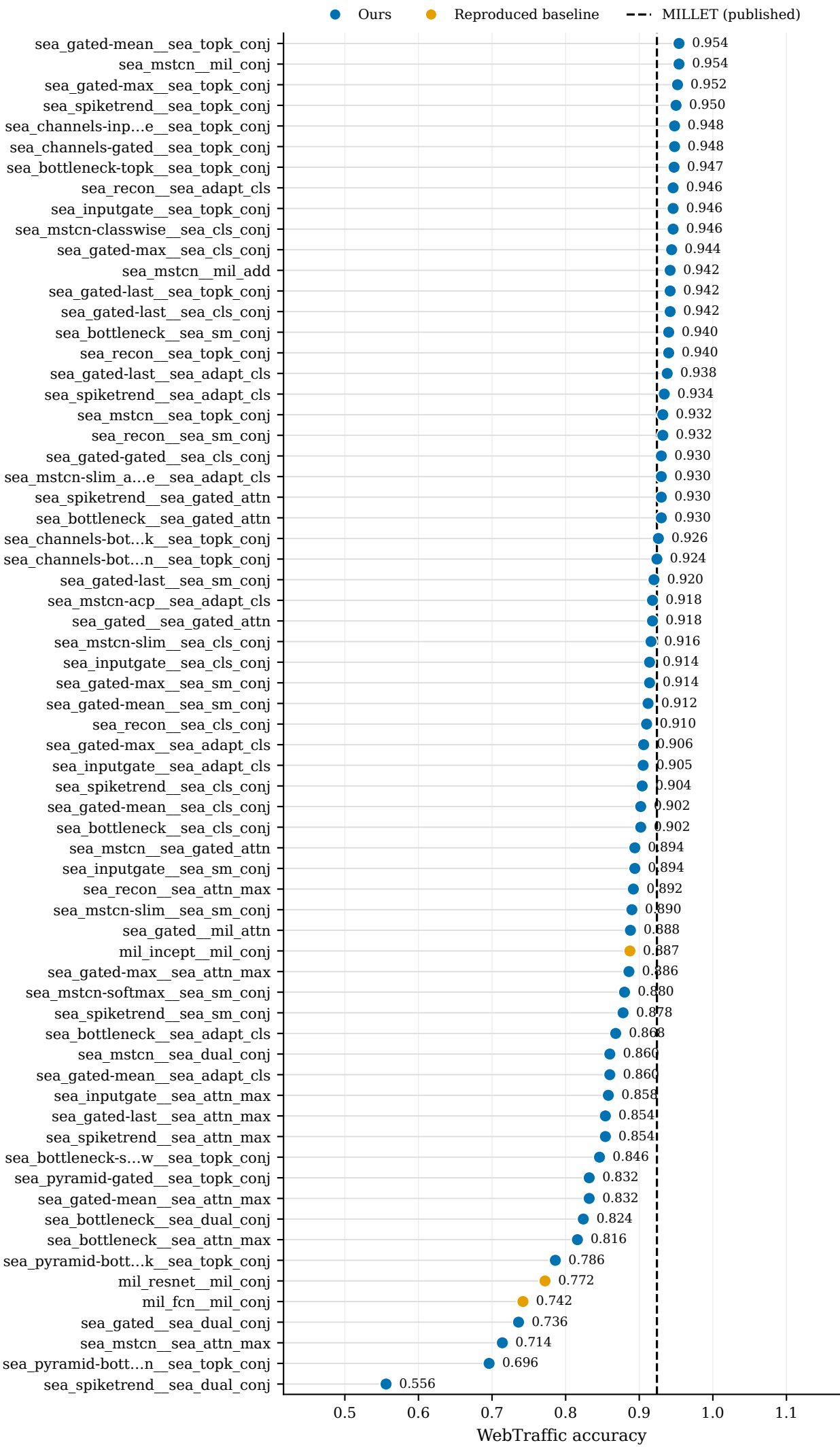
WebTraffic: Accuracy (all 66 models)
