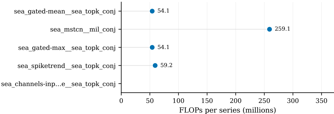
Top-5: FLOPs
