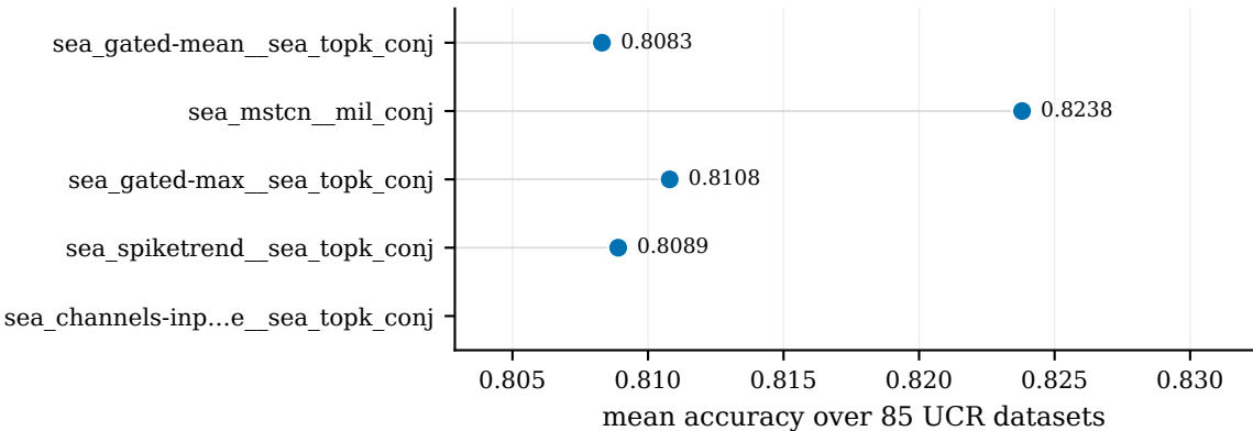
Top-5: UCR-85 accuracy
