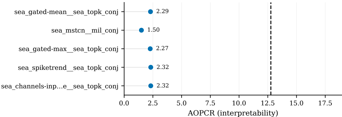
Top-5: AOPCR
