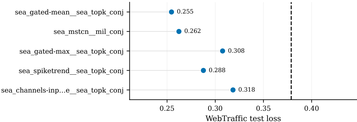
Top-5: Loss
