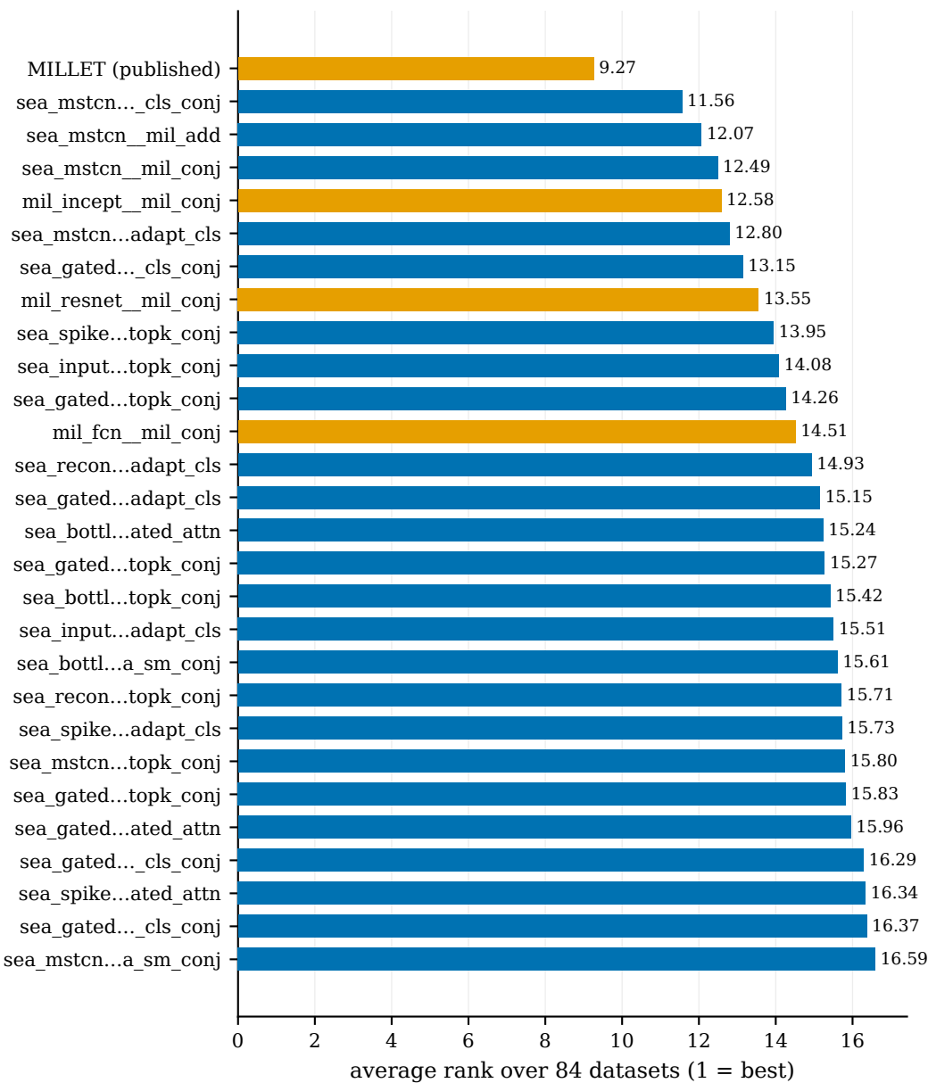
Average rank (accuracy)
