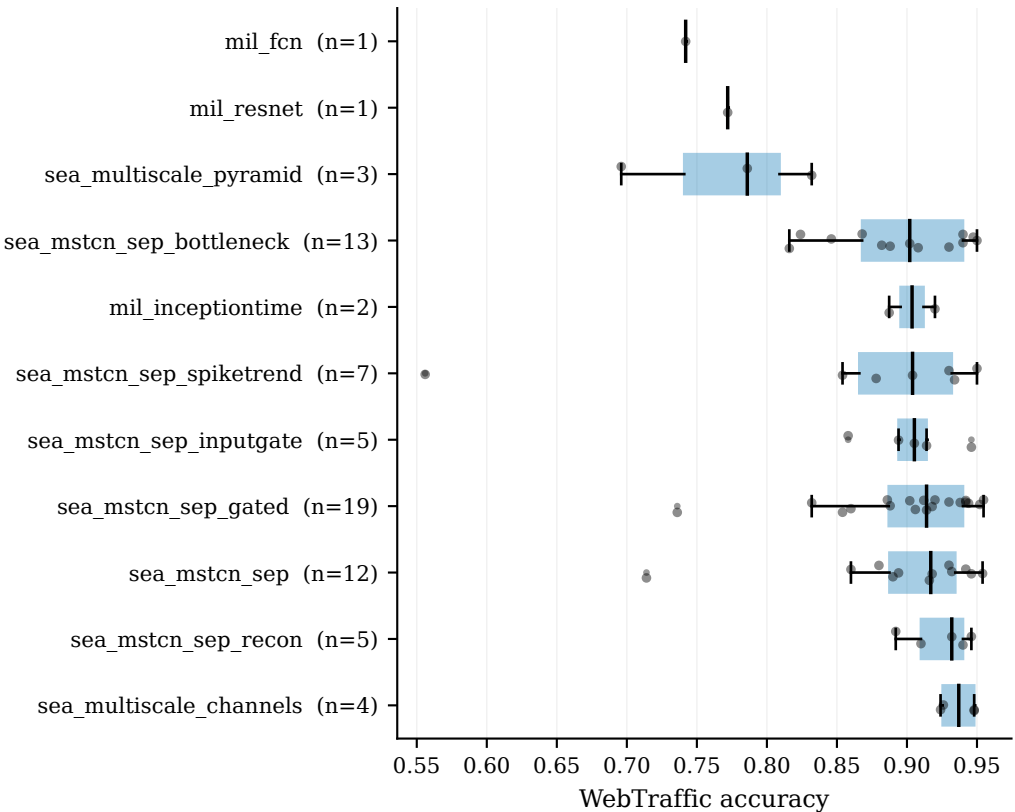
Accuracy by encoder (pooling head varies within each group)
