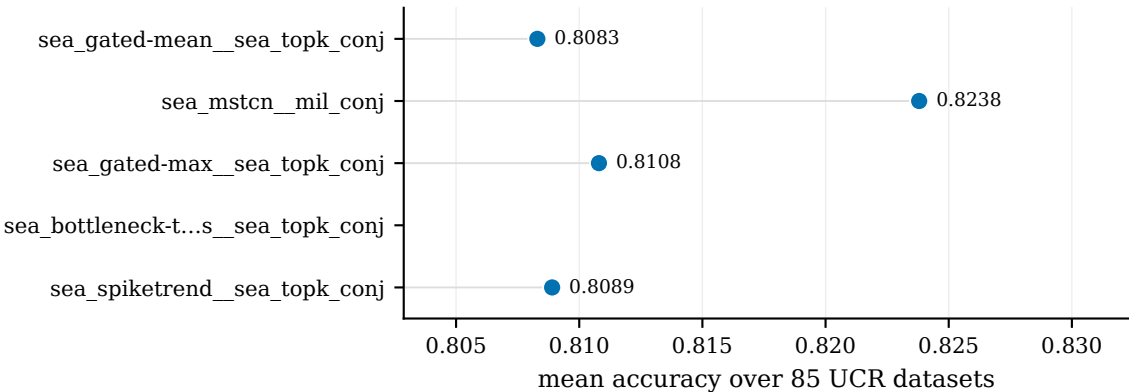
Top-5: UCR-85 accuracy
