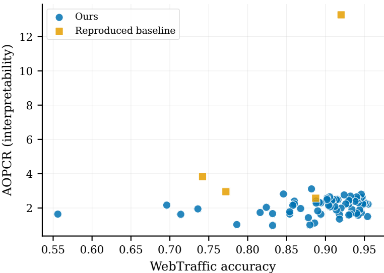
Accuracy vs AOPCR (Spearman \rho = 0.18 )
