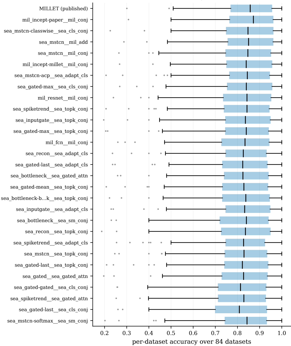
Distribution of accuracy across datasets
