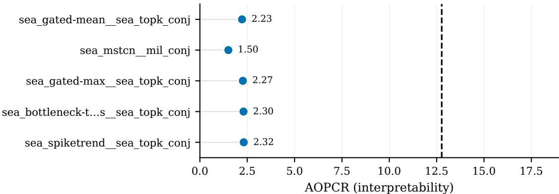
Top-5: AOPCR
