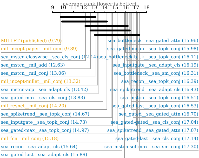
Critical difference diagram - accuracy over 84 datasets 29 models, Wilcoxon signed-rank with Holm correction ( \alpha=0.05 )
