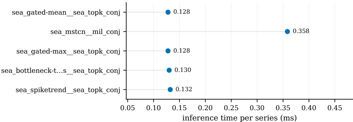
Top-5: Inference time
