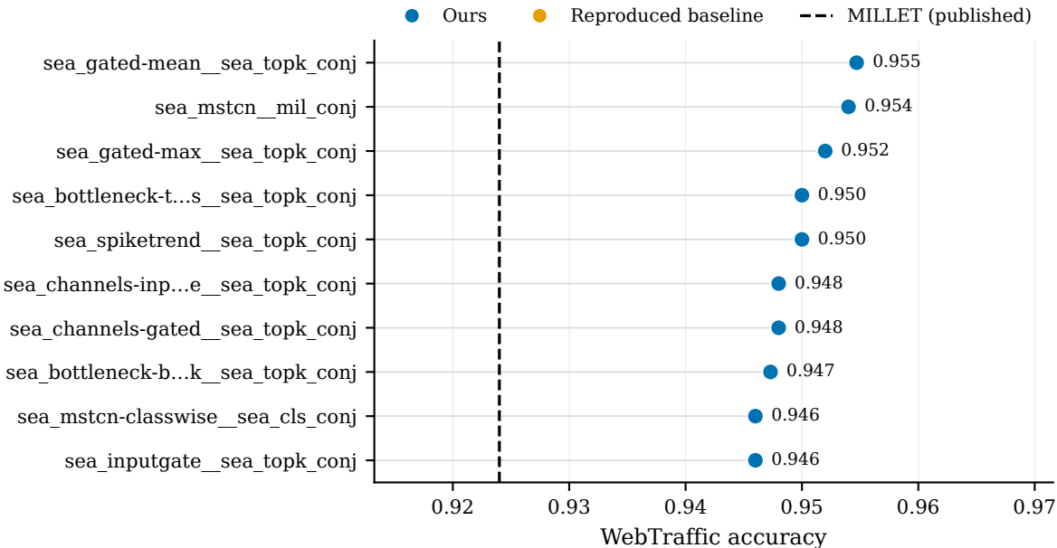
WebTraffic: Accuracy (top 10)
