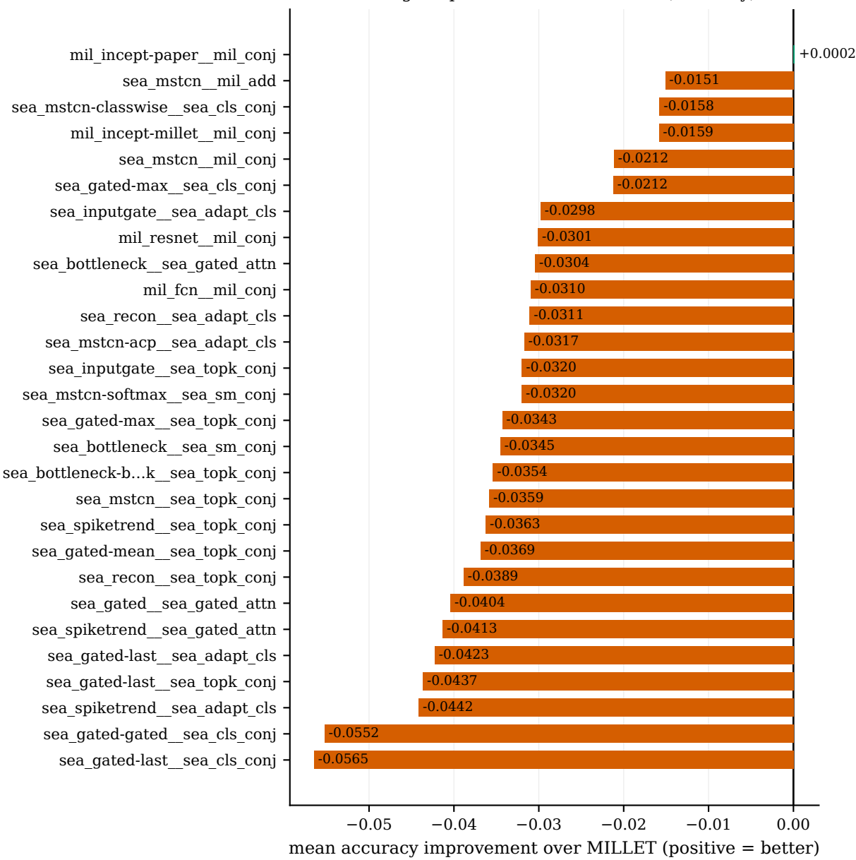
Average improvement over MILLET (accuracy)
