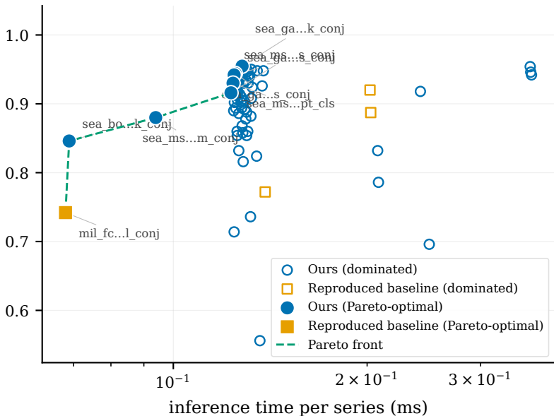
Accuracy vs Inference time
