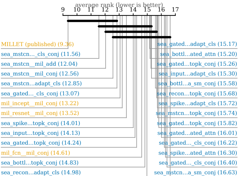
Critical difference diagram - accuracy over 84 datasets 28 models, Wilcoxon signed-rank with Holm correction ( \alpha=0.05 )
