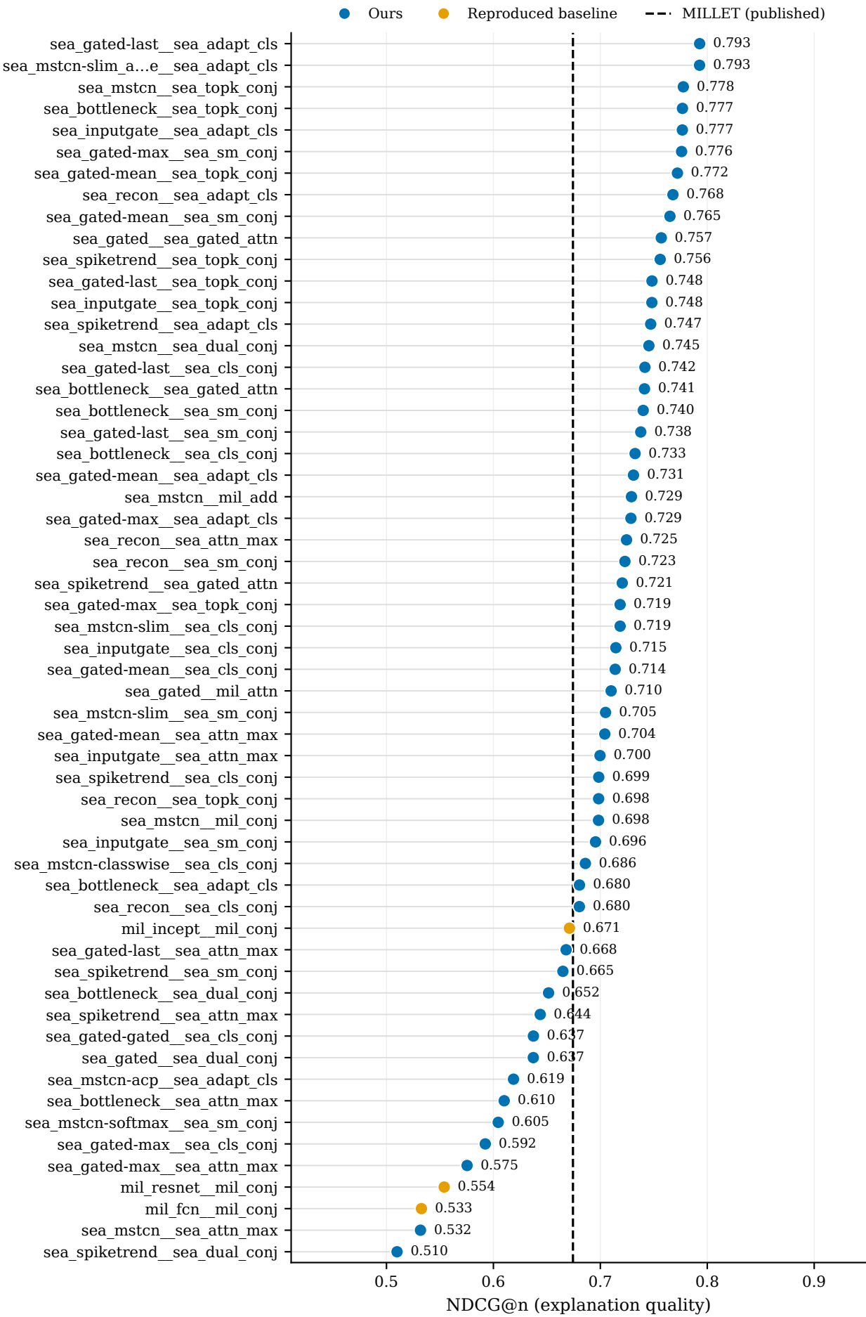
WebTraffic: NDCG@n (all 57 models)
