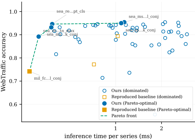
Accuracy vs Inference time
