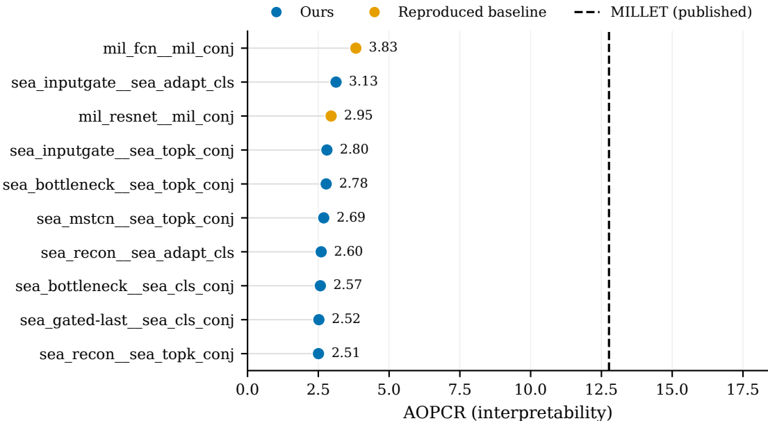
WebTraffic: AOPCR (top 10)
