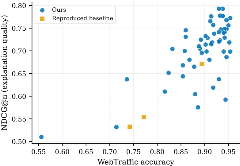
Accuracy vs NDCG@n (Spearman \rho = 0.60 )
