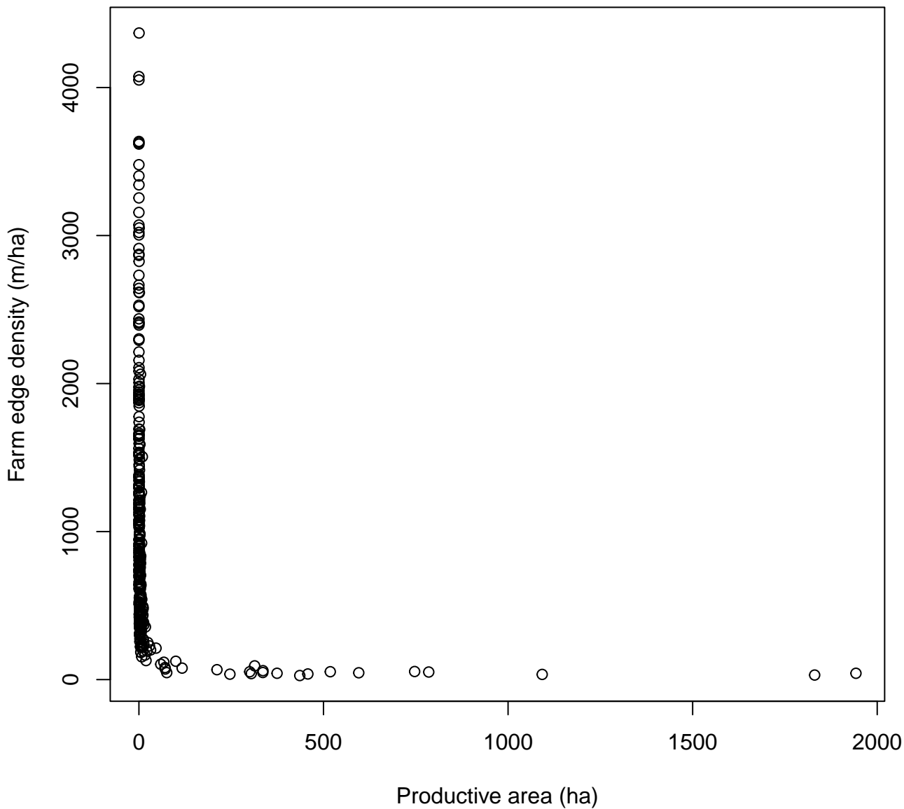
Productive area vs edge density
