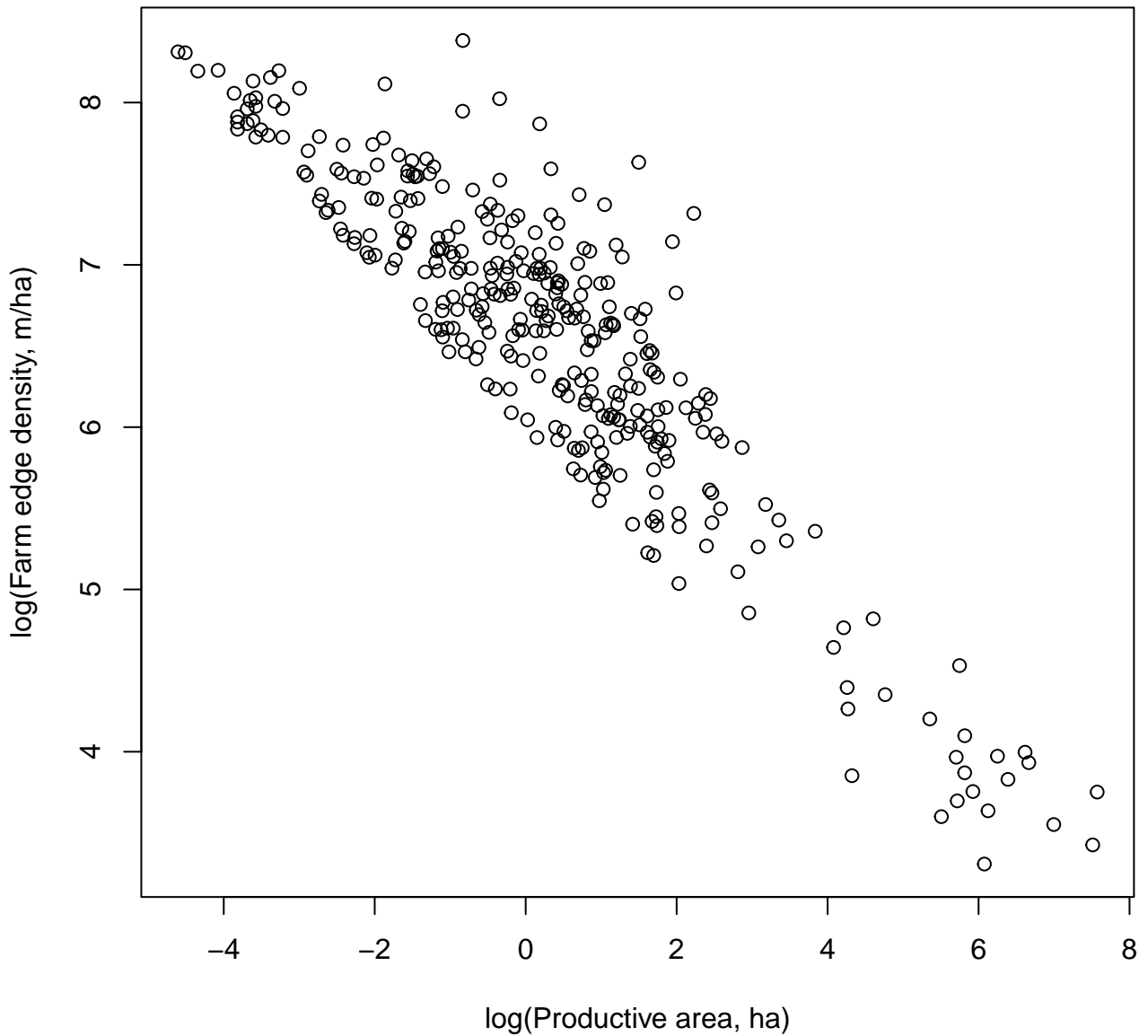
ln(Productive area) vs ln(Edge density)
