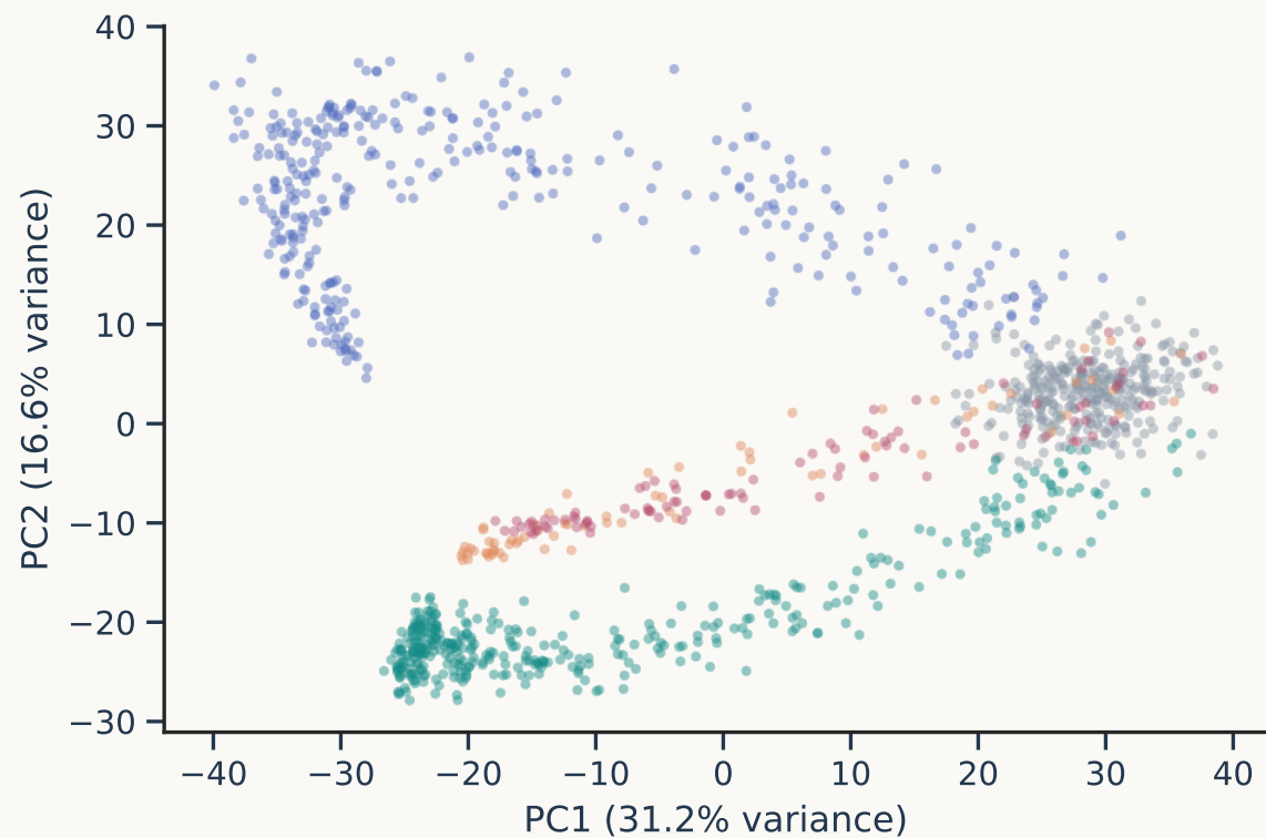
Centered rates without standardization
