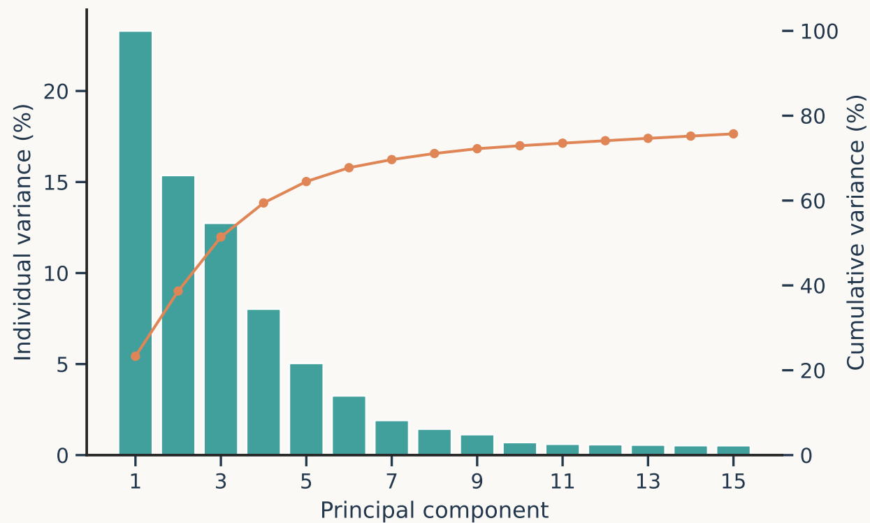
Standardized PCA: explained variance
