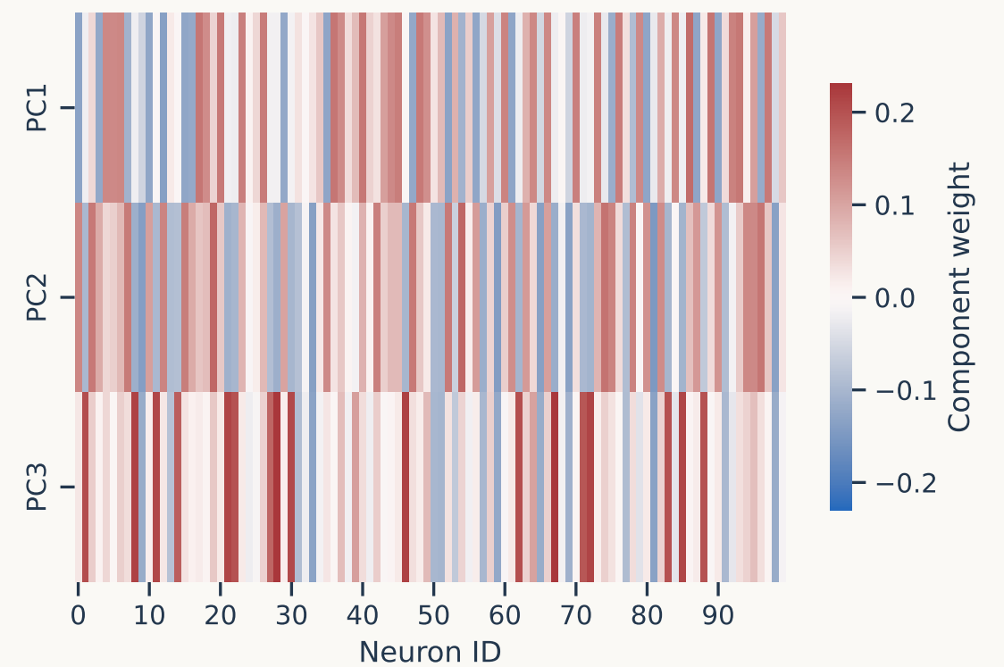
Standardized PCA: signed neuron weights
