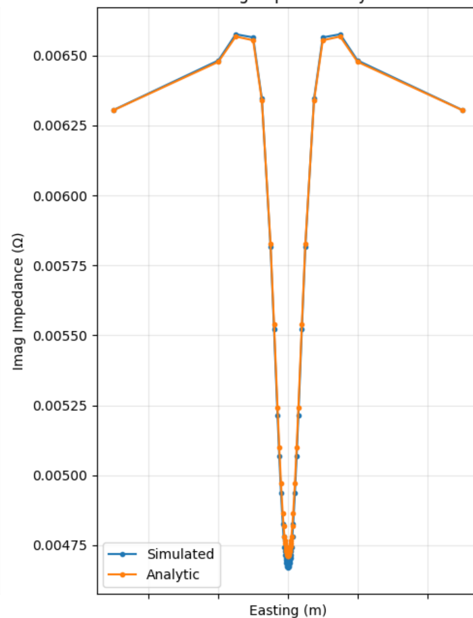
Apparent Resistivity, Phase, and Impedance along Cut at y=0 for 0.01Hz
