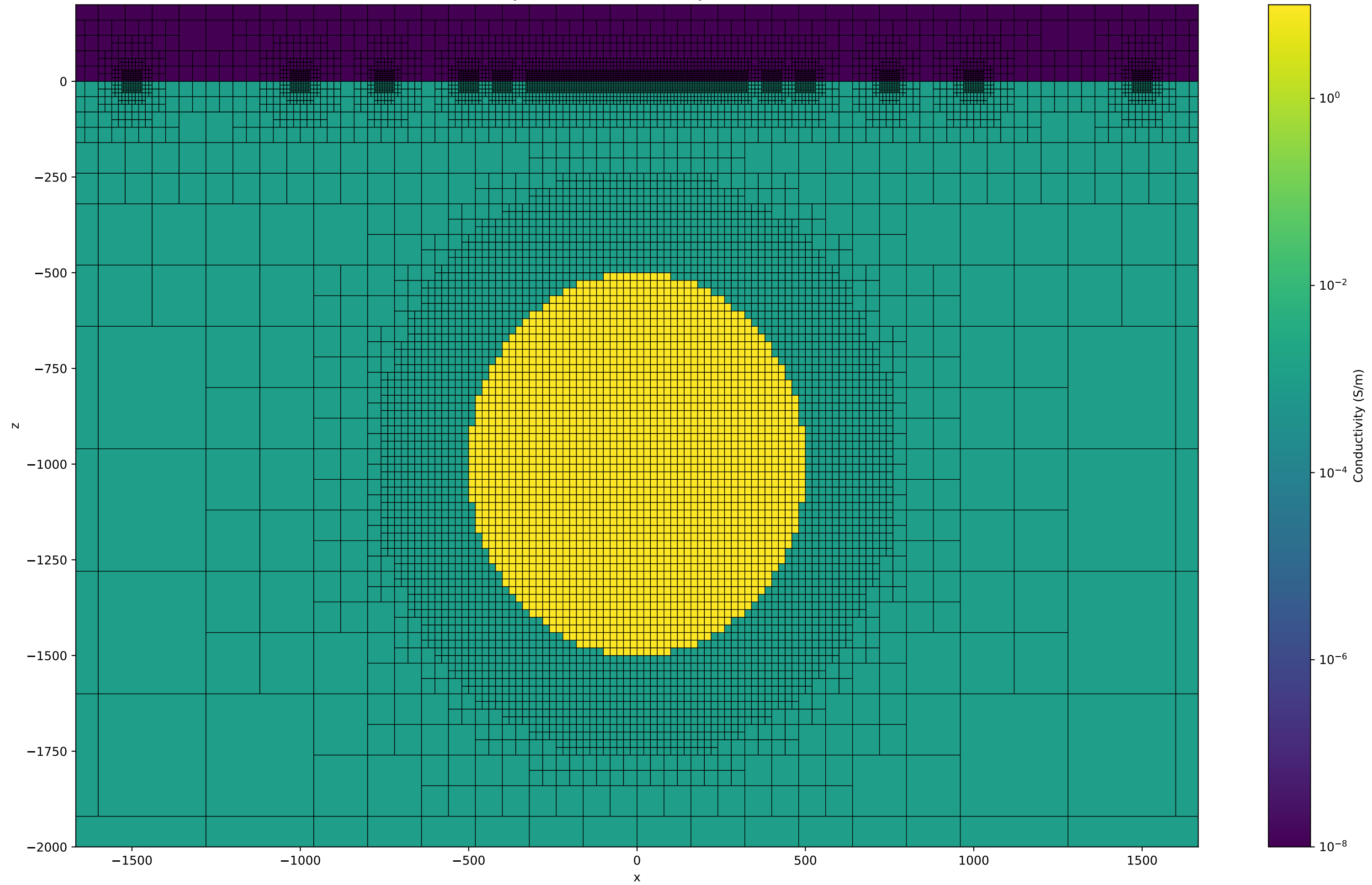
Mesh 6, Simulated in 3.00 hours Conductivity Model Cross Section at y=0, 2,206,548 cells
