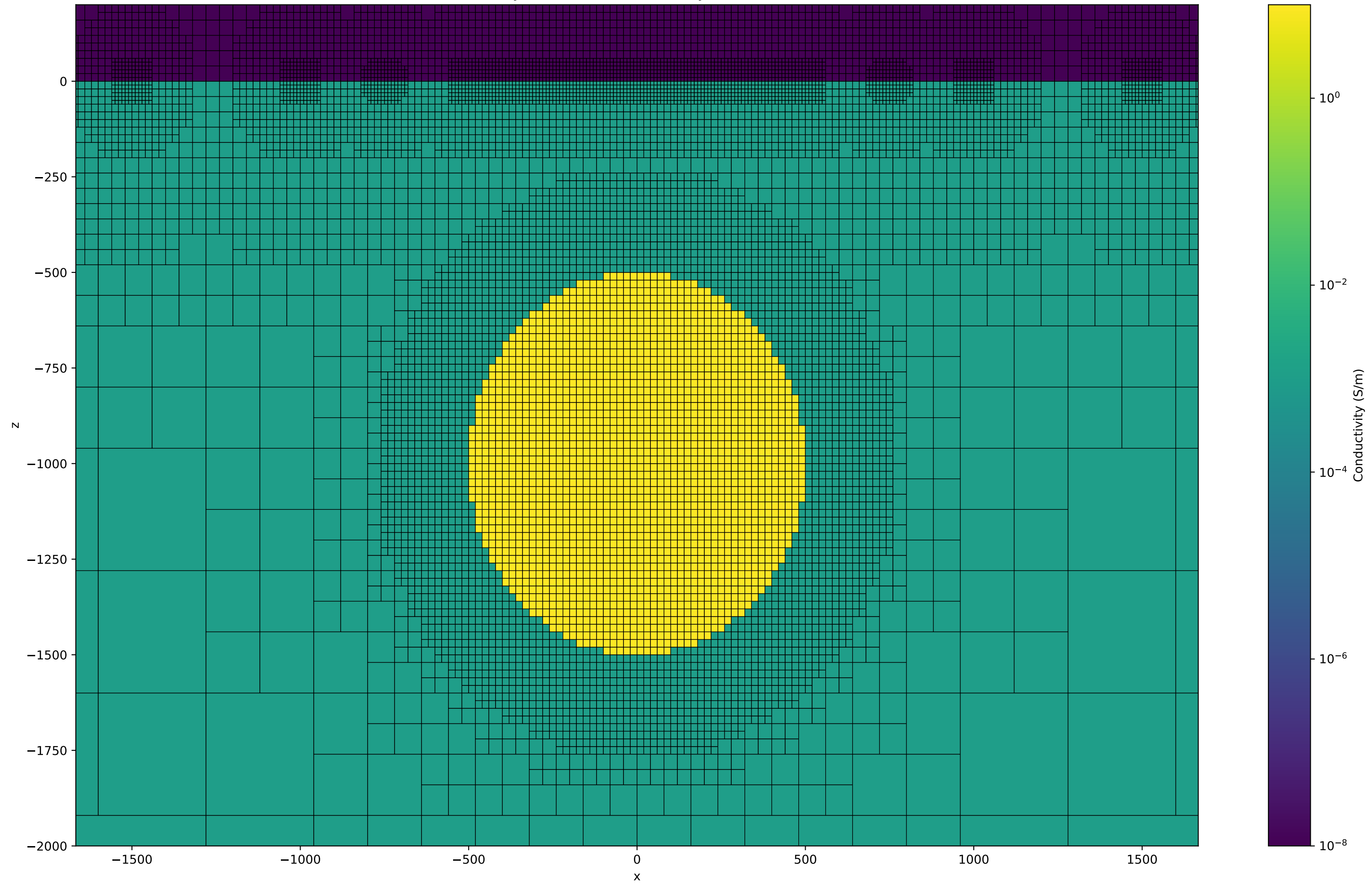
Mesh 7, Simulated in 6.38 hours Conductivity Model Cross Section at y=0, 2,243,536 cells
