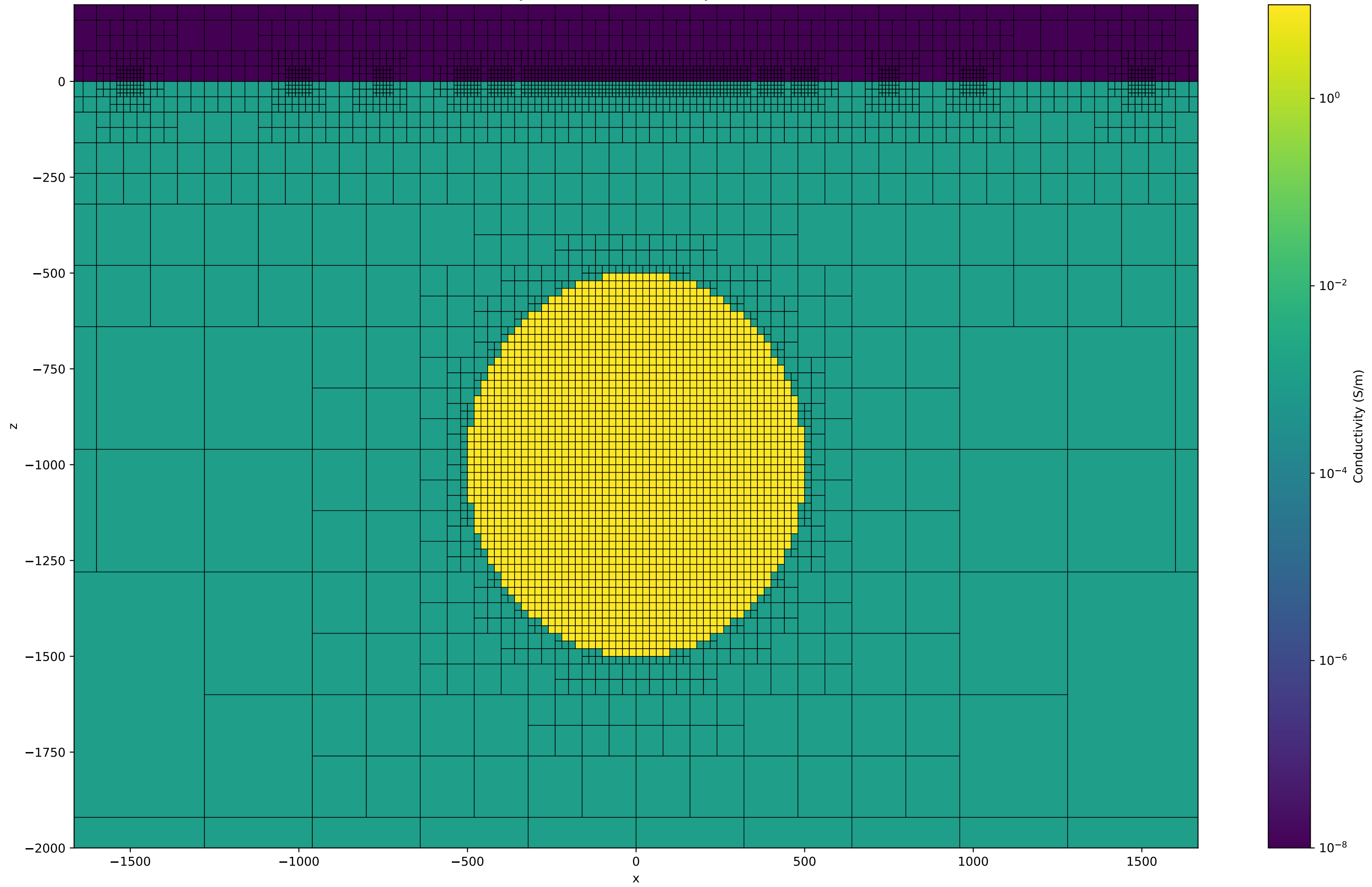
Mesh 2, Simulated in 0.57 hours Conductivity Model Cross Section at y=0, 788,292 cells
