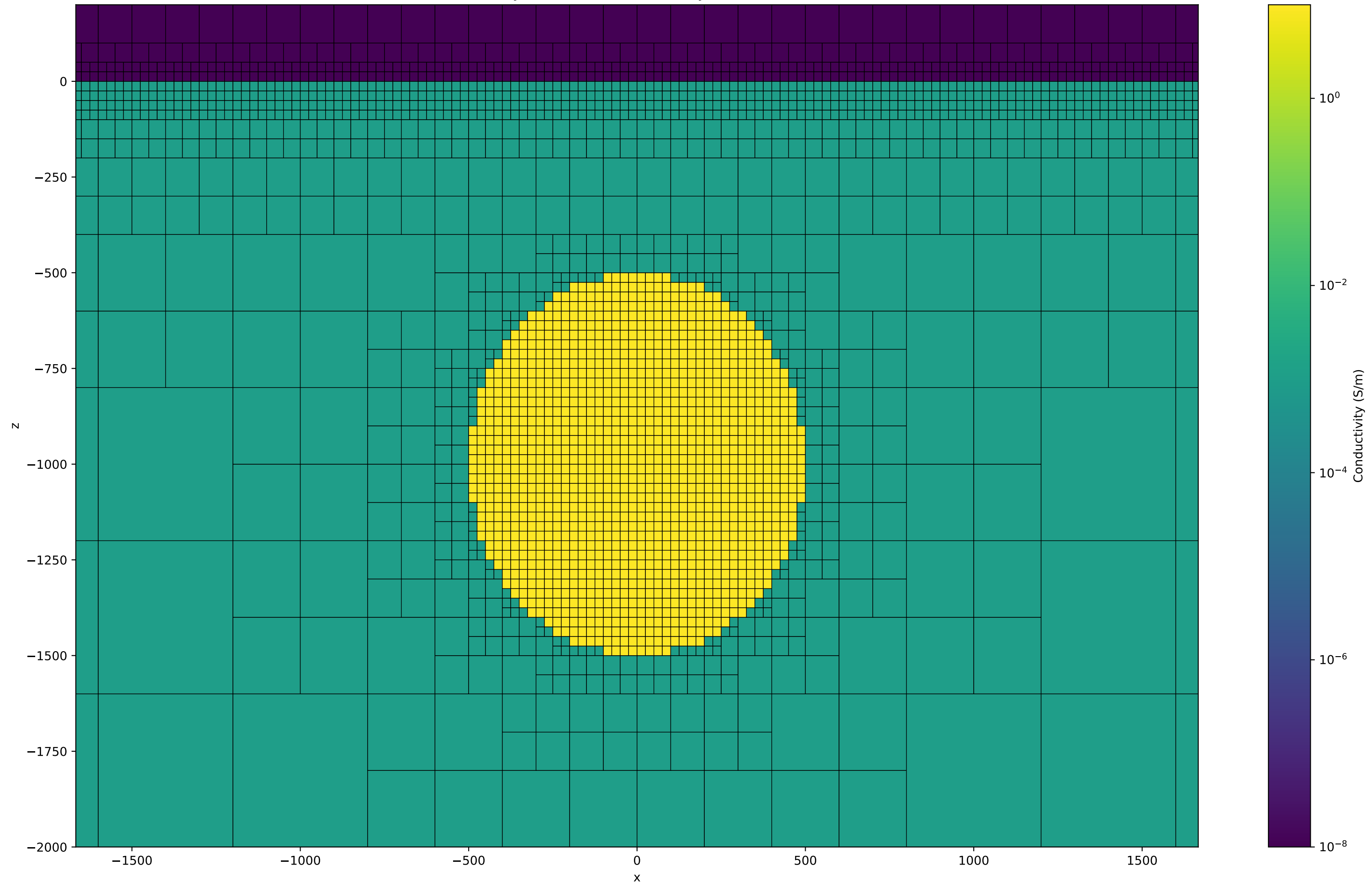
Mesh 4, Simulated in 1.89 hours Conductivity Model Cross Section at y=0 , 1,208,404 cells
