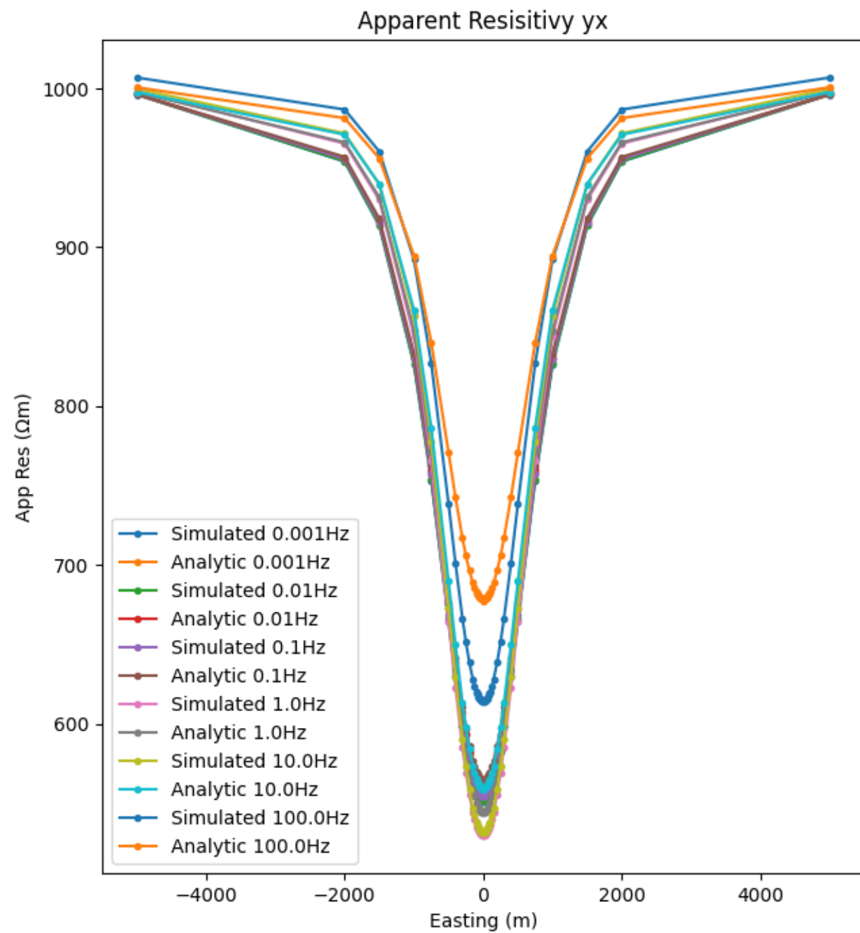
yx Apparent Resistivity and Phase along Cut at y=0
