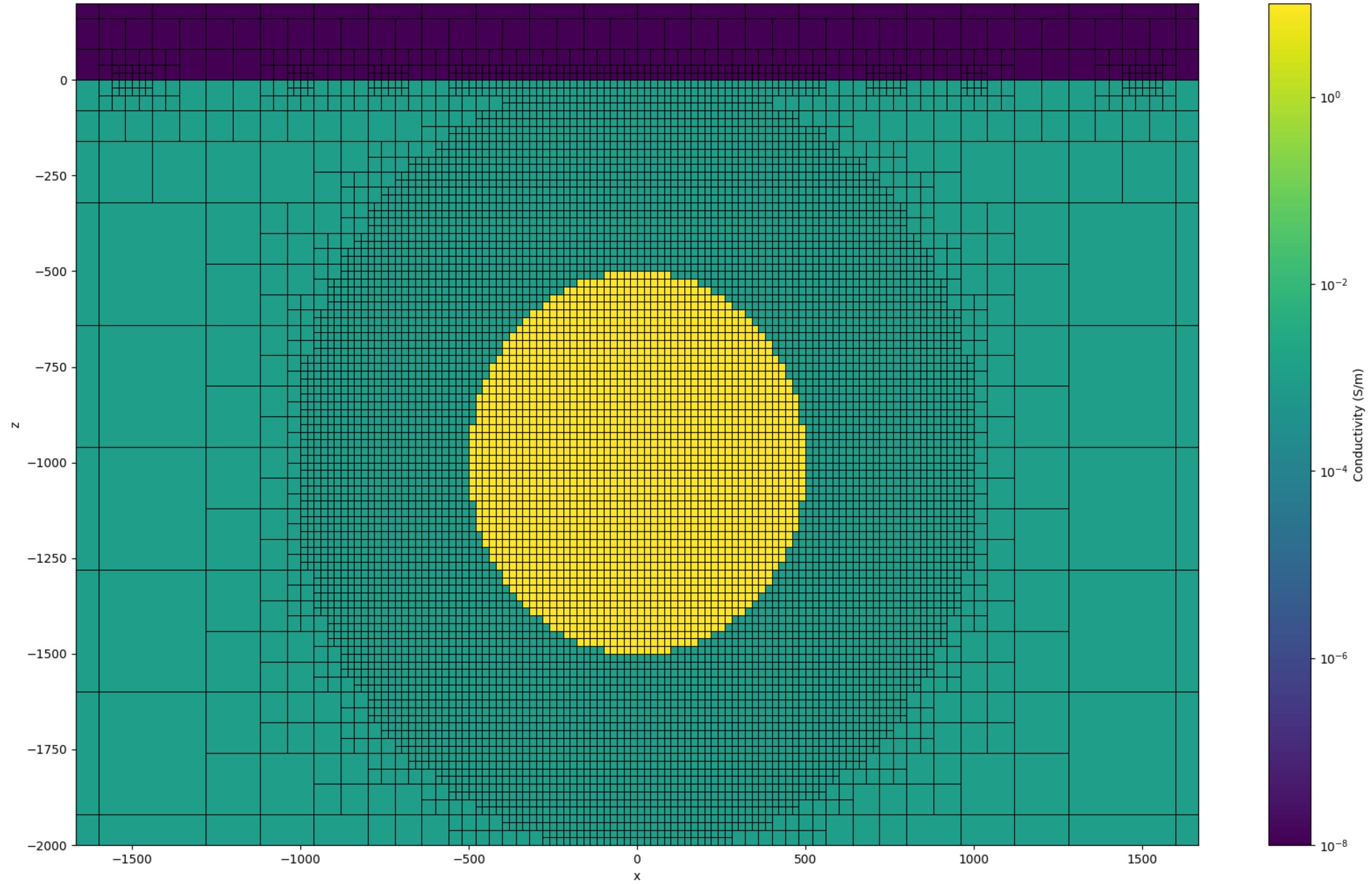
Conductivity Model Cross Section at y=0, 763764 cells
