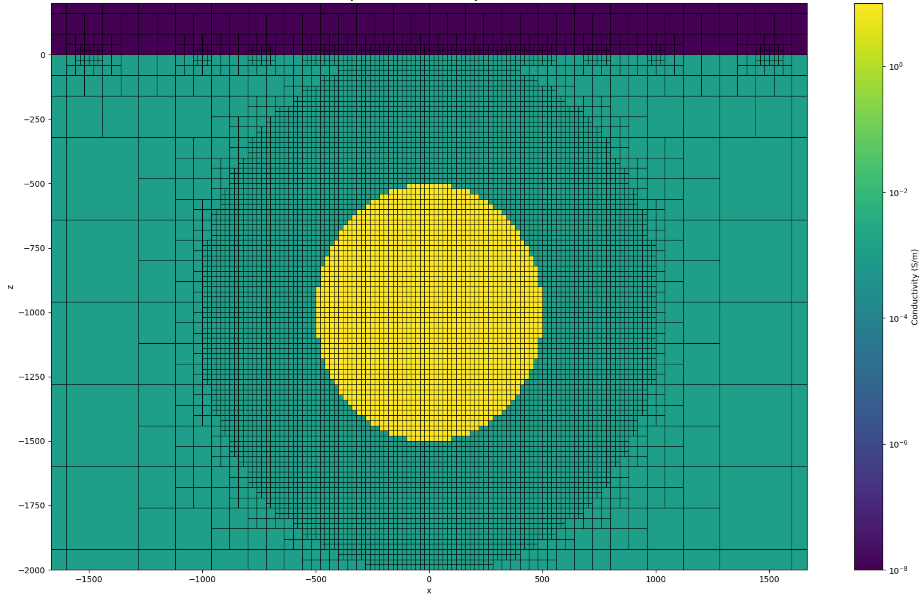
Mesh 1, Simulated in 8.87 hours Conductivity Model Cross Section at y=0 , 763,764 cells
