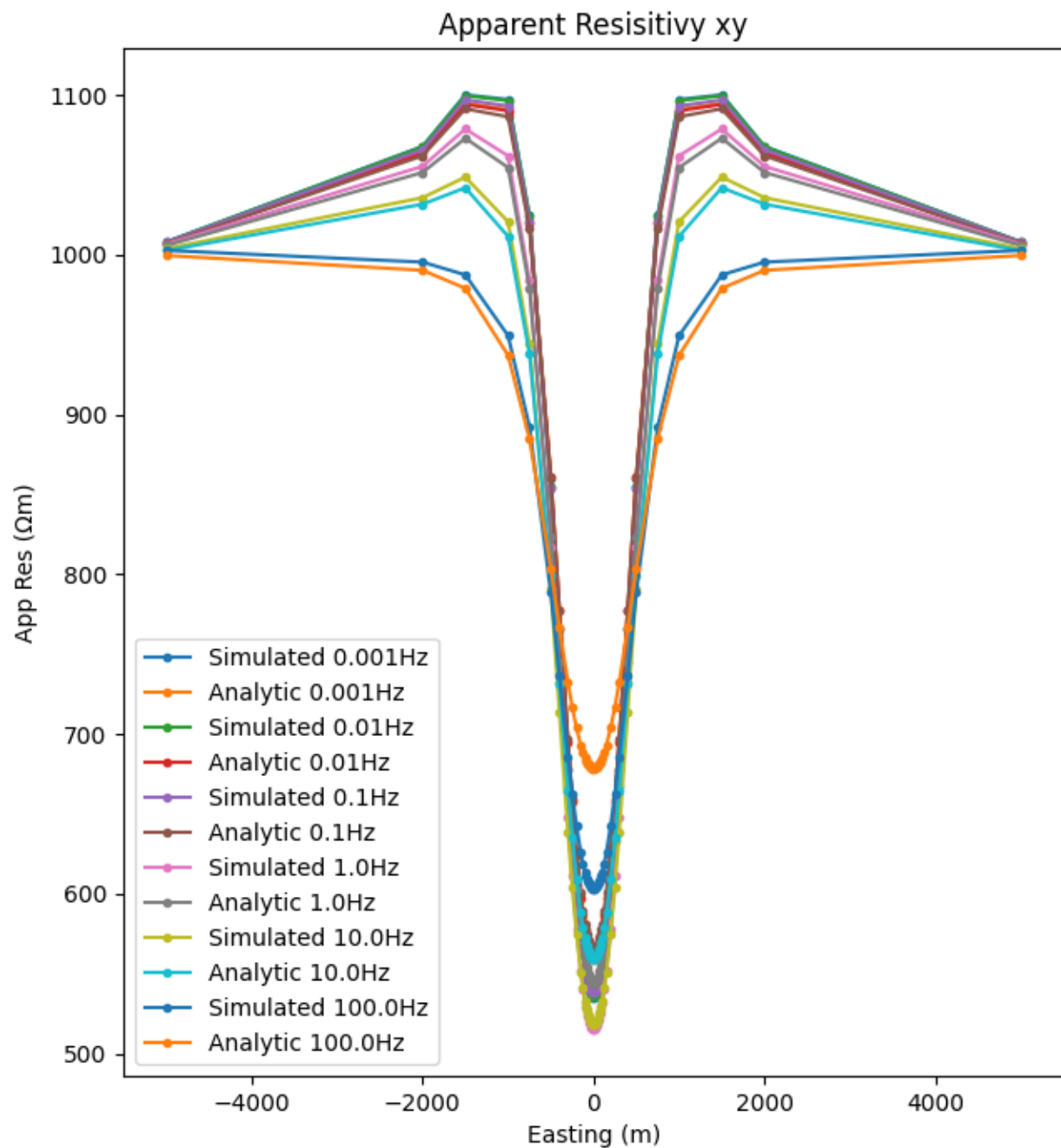
xy Apparent Resistivity and Phase along Cut at y=0
