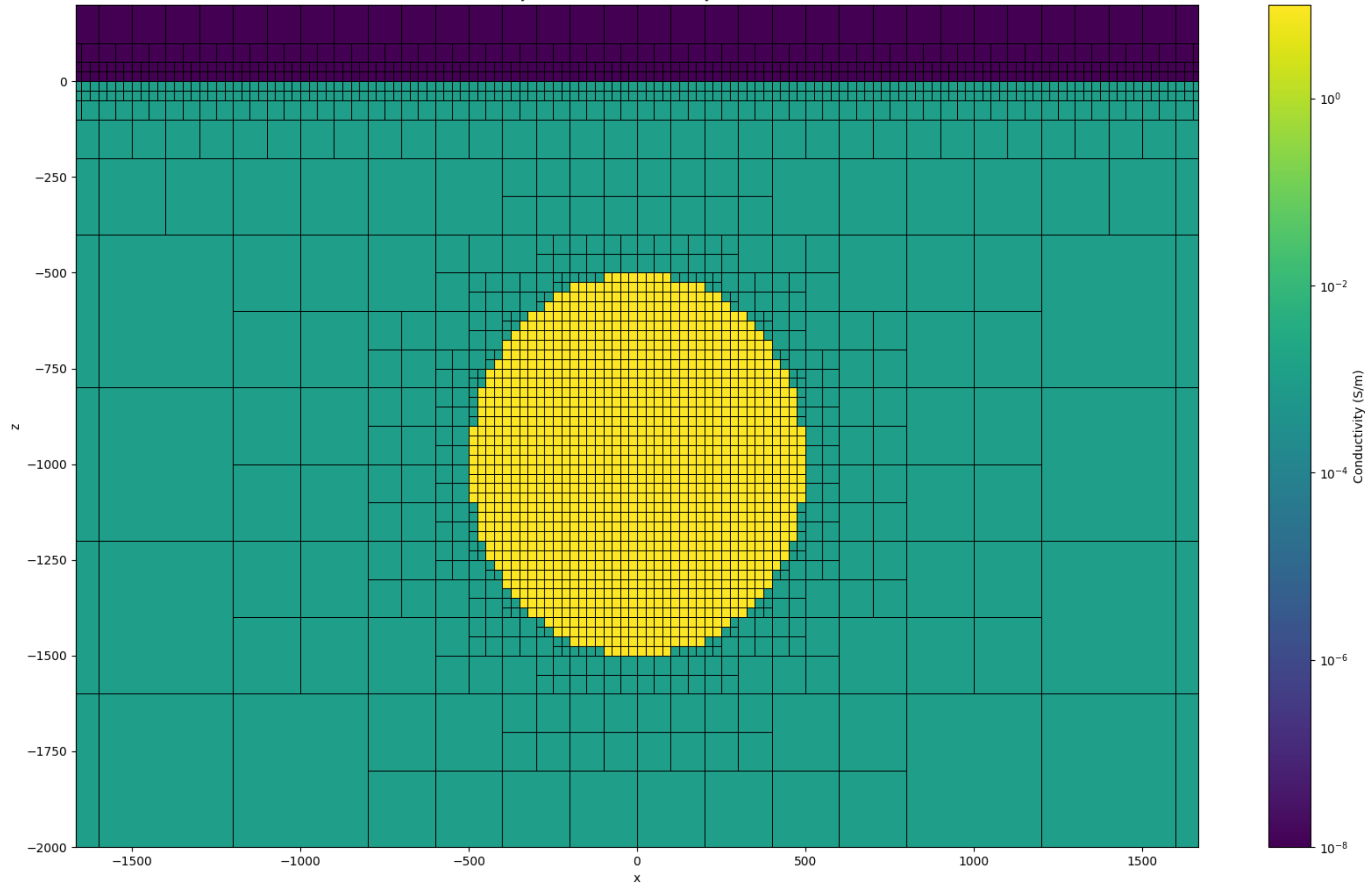
Mesh 3, Simulated in 0.51 hours Conductivity Model Cross Section at y=0 , 825,196 cells
