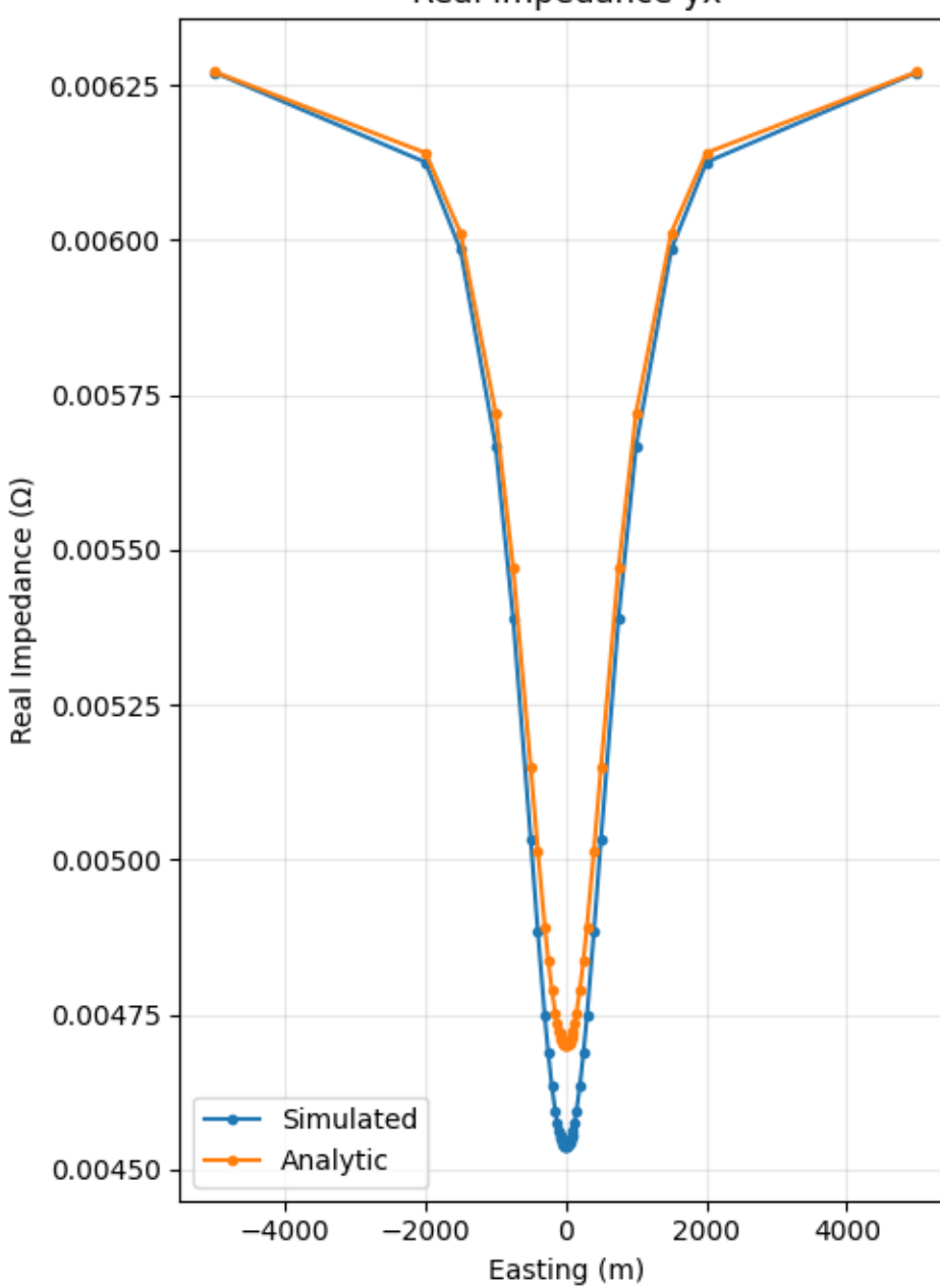
Real Impedance yx
