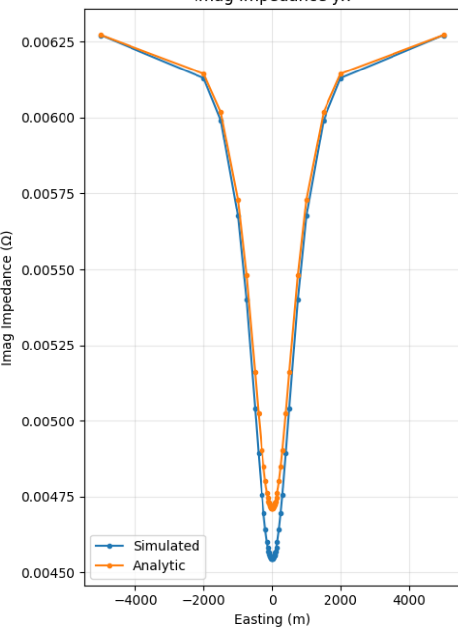
Imag Impedance yx
