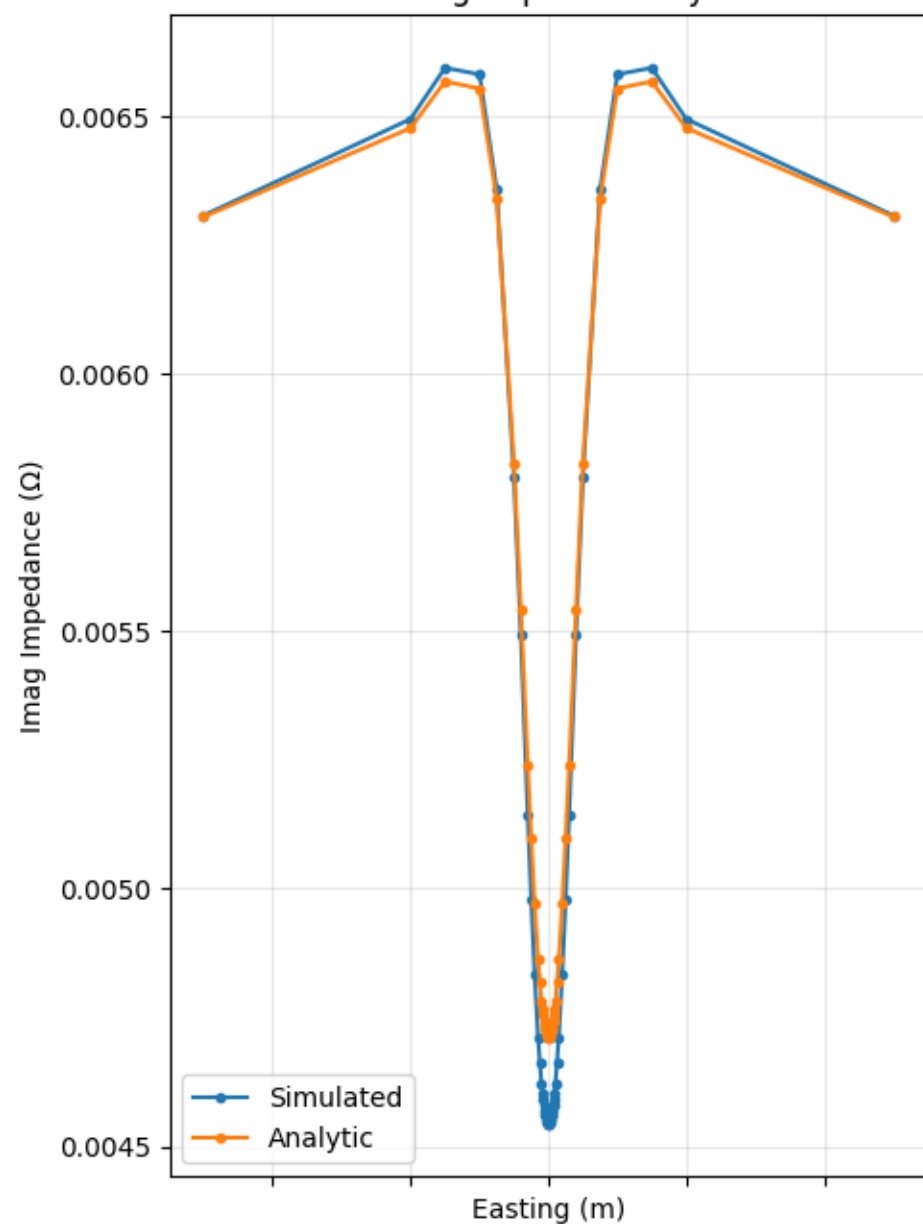
Imag Impedance yx
