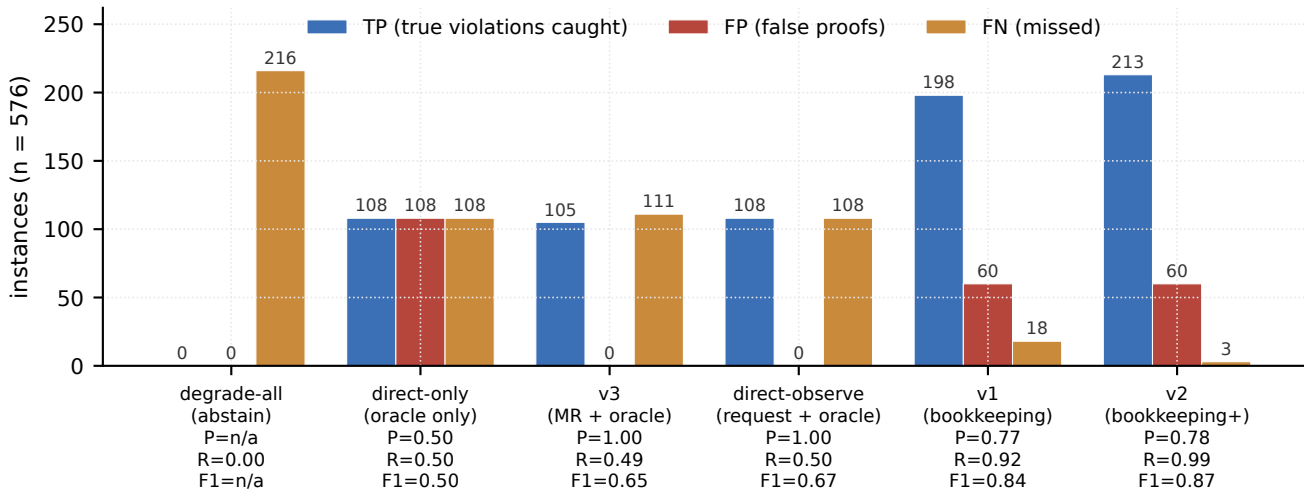
Adjudicator comparison: the MR trigger does not carry the work (Block 9, synthetic matrix)
