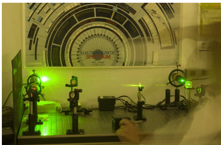
Figure 5. Immobileyes electro-optics/laser laboratory (Kent, OH)—optical benches and multi-wavelength laser sources for the Phase I test campaign.
