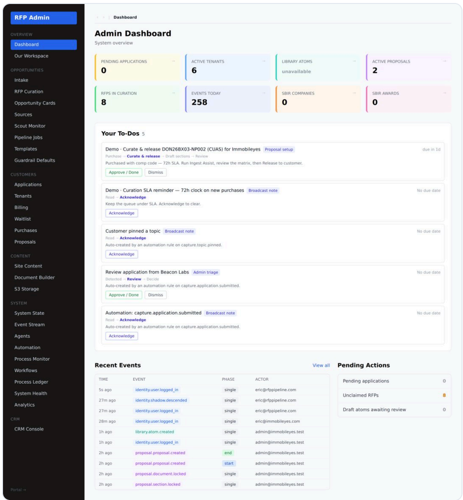
The admin Dashboard — stat tiles, ToDos, recent events, pending actions.
