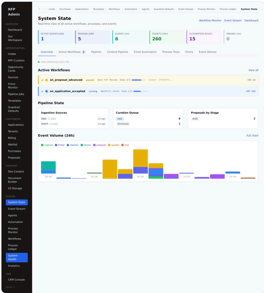
System State — HealthBar + eight tabs (Overview, Workflows, Pipeline, Content, Email, Trees, Errors, Volume).
