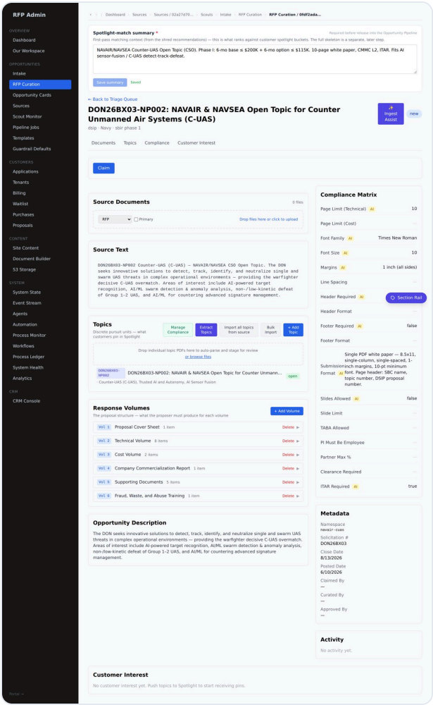
The curation workspace — documents, PDF tagging, topics, volumes, compliance matrix.
